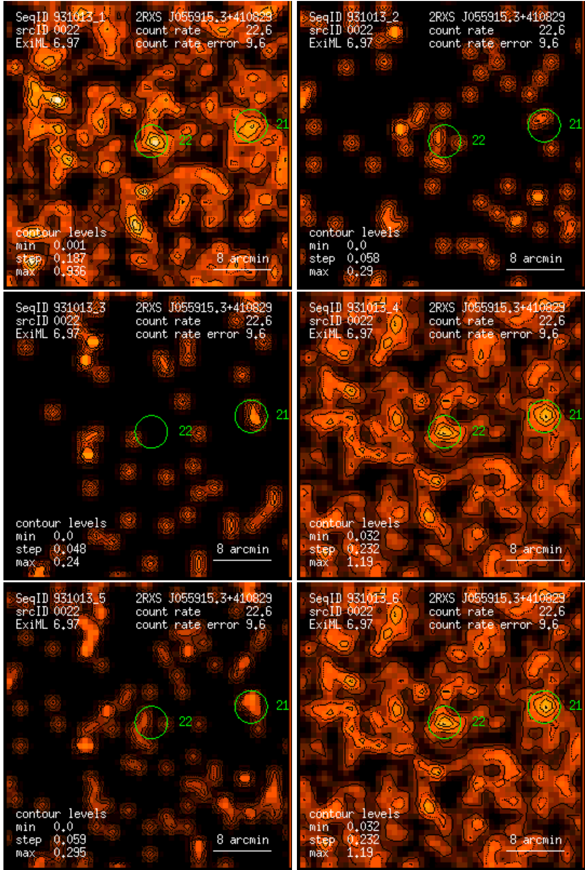
Figure 22: RASS 931013: detection 0022: band rate images, Gaussian filter: (1) PSPC channels 11 – 41, (2) 52 – 90, (3) 91 – 201, (4) 11 – 235, (5) 52 – 201, (6) 11 – 201. Broad band rates in counts/ks. Band rate contour levels in counts/ks/arcmin 2 .
