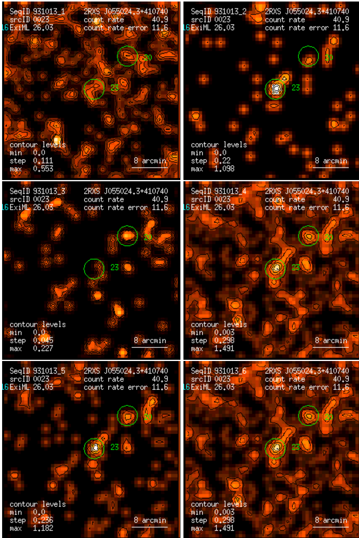
Figure 23: RASS 931013: detection 0023: band rate images, Gaussian filter: (1) PSPC channels 11 – 41, (2) 52 – 90, (3) 91 – 201, (4) 11 – 235, (5) 52 – 201, (6) 11 – 201. Broad band rates in counts/ks. Band rate contour levels in counts/ks/arcmin 2 .
