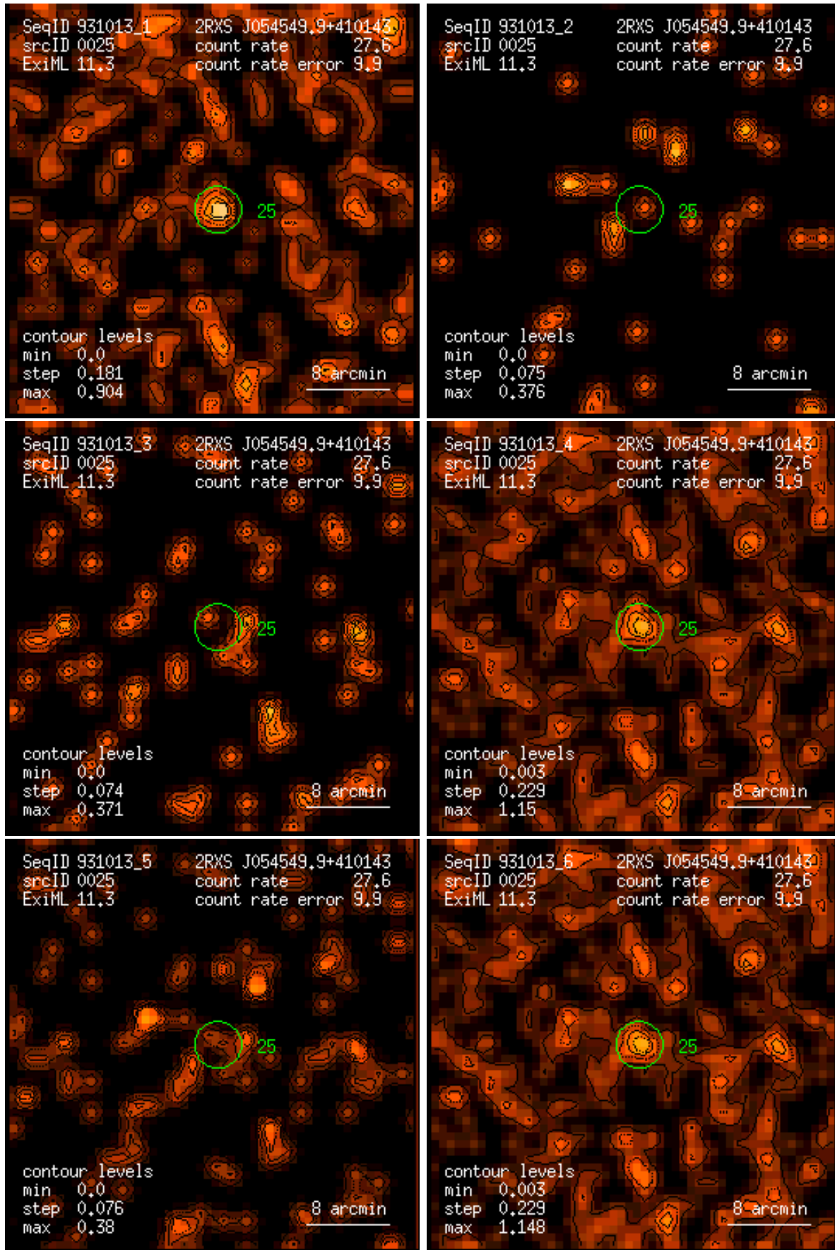
Figure 25: RASS 931013: detection 0025: band rate images, Gaussian filter: (1) PSPC channels 11 – 41, (2) 52 – 90, (3) 91 – 201, (4) 11 – 235, (5) 52 – 201, (6) 11 – 201. Broad band rates in counts/ks. Band rate contour levels in counts/ks/arcmin 2 .
