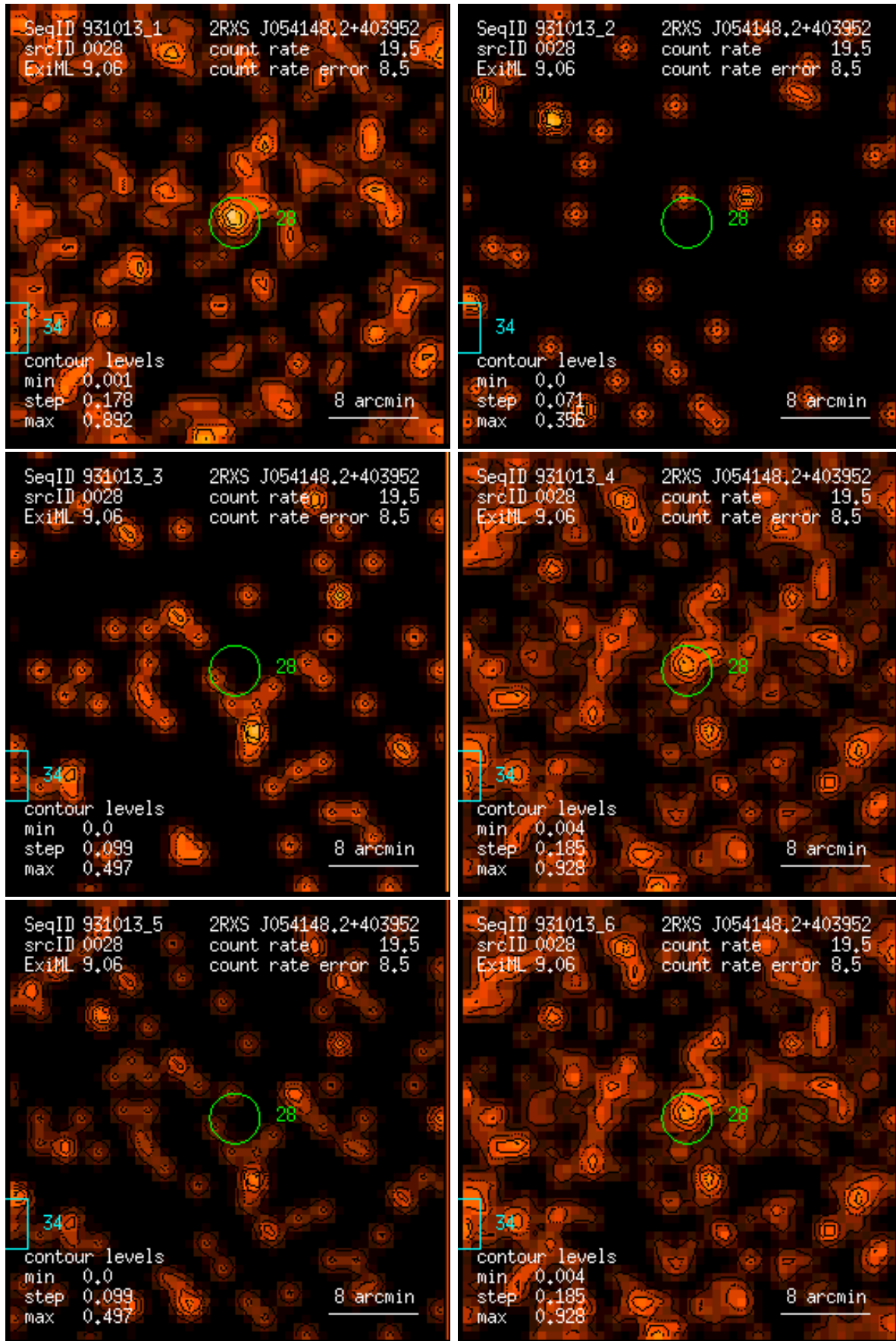
Figure 28: RASS 931013: detection 0028: band rate images, Gaussian filter: (1) PSPC channels 11 – 41, (2) 52 – 90, (3) 91 – 201, (4) 11 – 235, (5) 52 – 201, (6) 11 – 201. Broad band rates in counts/ks. Band rate contour levels in counts/ks/arcmin 2 .
