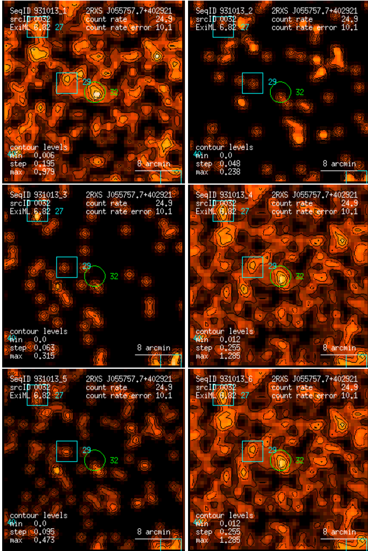
Figure 32: RASS 931013: detection 0032: band rate images, Gaussian filter: (1) PSPC channels 11 – 41, (2) 52 – 90, (3) 91 – 201, (4) 11 – 235, (5) 52 – 201, (6) 11 – 201. Broad band rates in counts/ks. Band rate contour levels in counts/ks/arcmin 2 .
