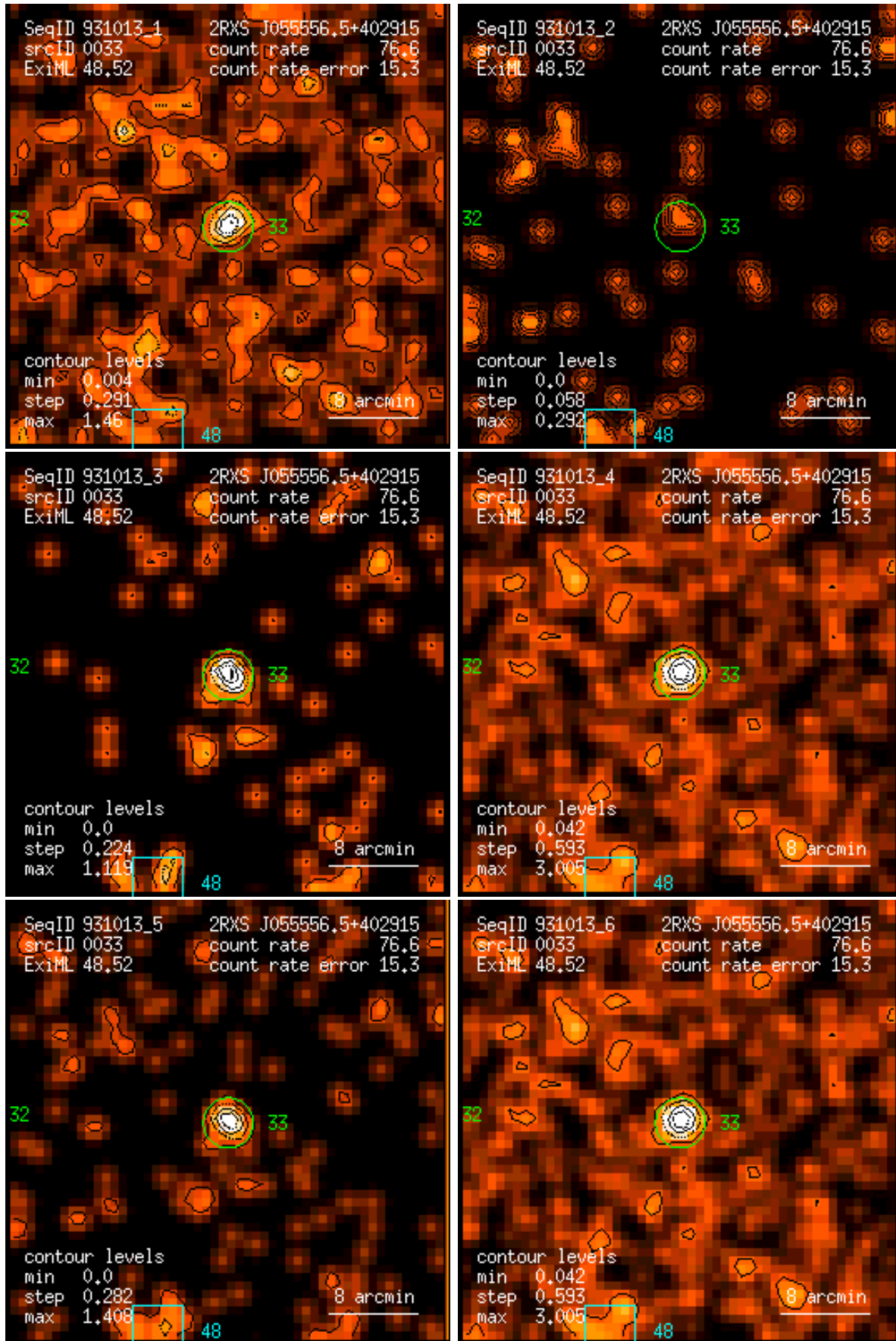
Figure 33: RASS 931013: detection 0033: band rate images, Gaussian filter: (1) PSPC channels 11 – 41, (2) 52 – 90, (3) 91 – 201, (4) 11 – 235, (5) 52 – 201, (6) 11 – 201. Broad band rates in counts/ks. Band rate contour levels in counts/ks/arcmin 2 .
