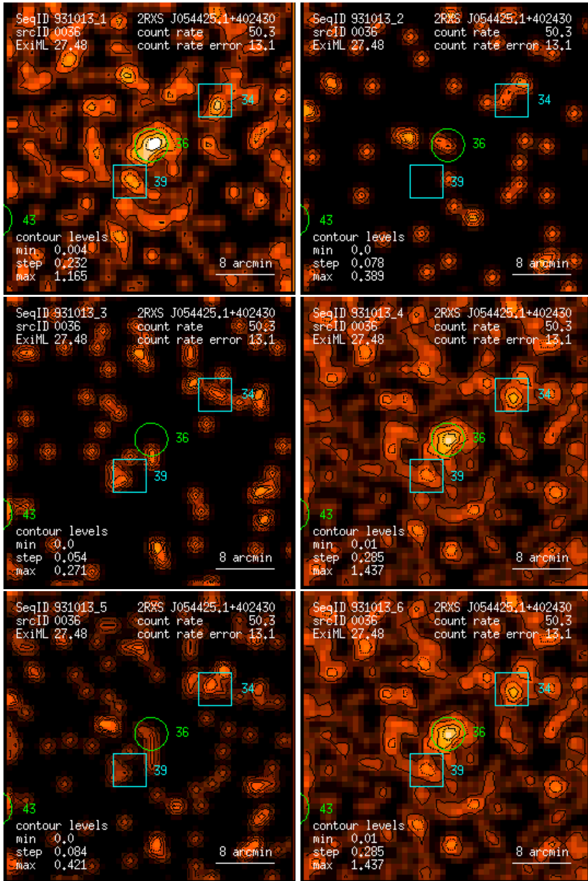
Figure 36: RASS 931013: detection 0036: band rate images, Gaussian filter: (1) PSPC channels 11 – 41, (2) 52 – 90, (3) 91 – 201, (4) 11 – 235, (5) 52 – 201, (6) 11 – 201. Broad band rates in counts/ks. Band rate contour levels in counts/ks/arcmin 2 .
