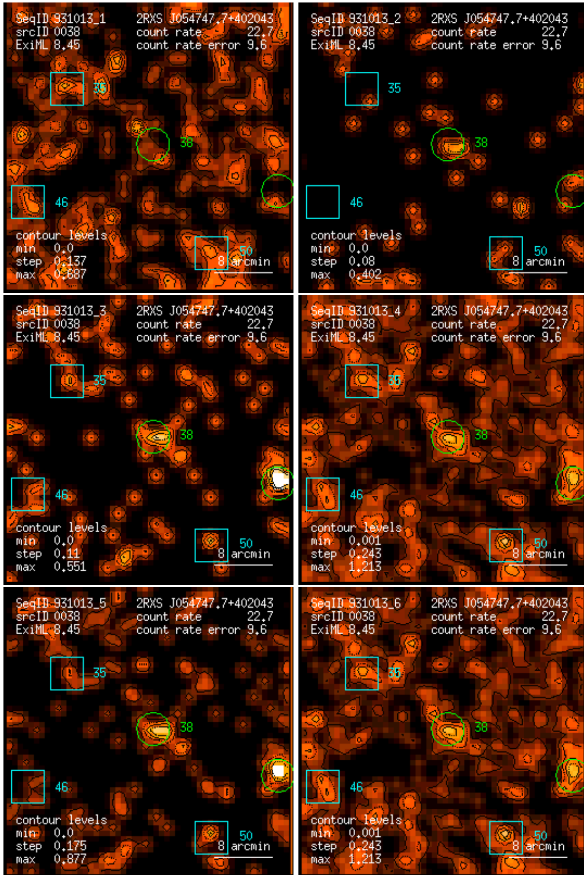
Figure 38: RASS 931013: detection 0038: band rate images, Gaussian filter: (1) PSPC channels 11 – 41, (2) 52 – 90, (3) 91 – 201, (4) 11 – 235, (5) 52 – 201, (6) 11 – 201. Broad band rates in counts/ks. Band rate contour levels in counts/ks/arcmin 2 .
