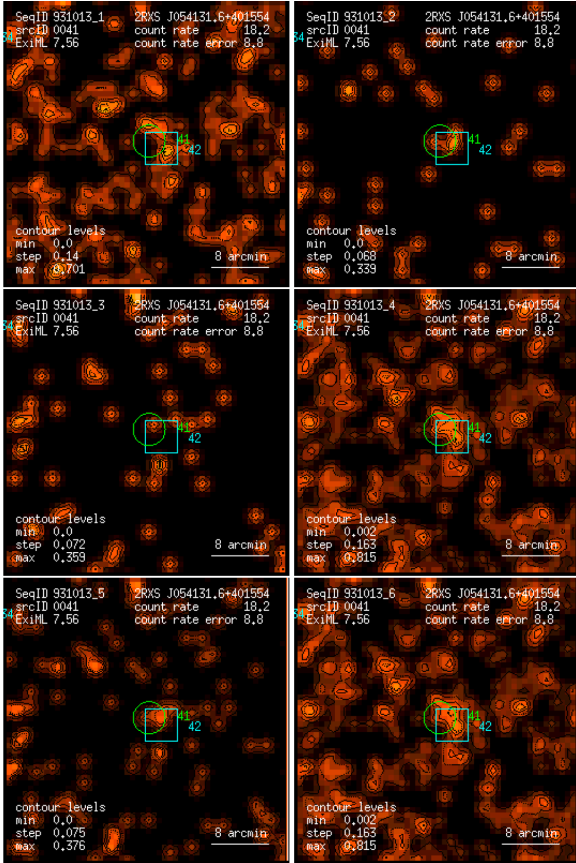
Figure 41: RASS 931013: detection 0041: band rate images, Gaussian filter: (1) PSPC channels 11 – 41, (2) 52 – 90, (3) 91 – 201, (4) 11 – 235, (5) 52 – 201, (6) 11 – 201. Broad band rates in counts/ks. Band rate contour levels in counts/ks/arcmin 2 .
