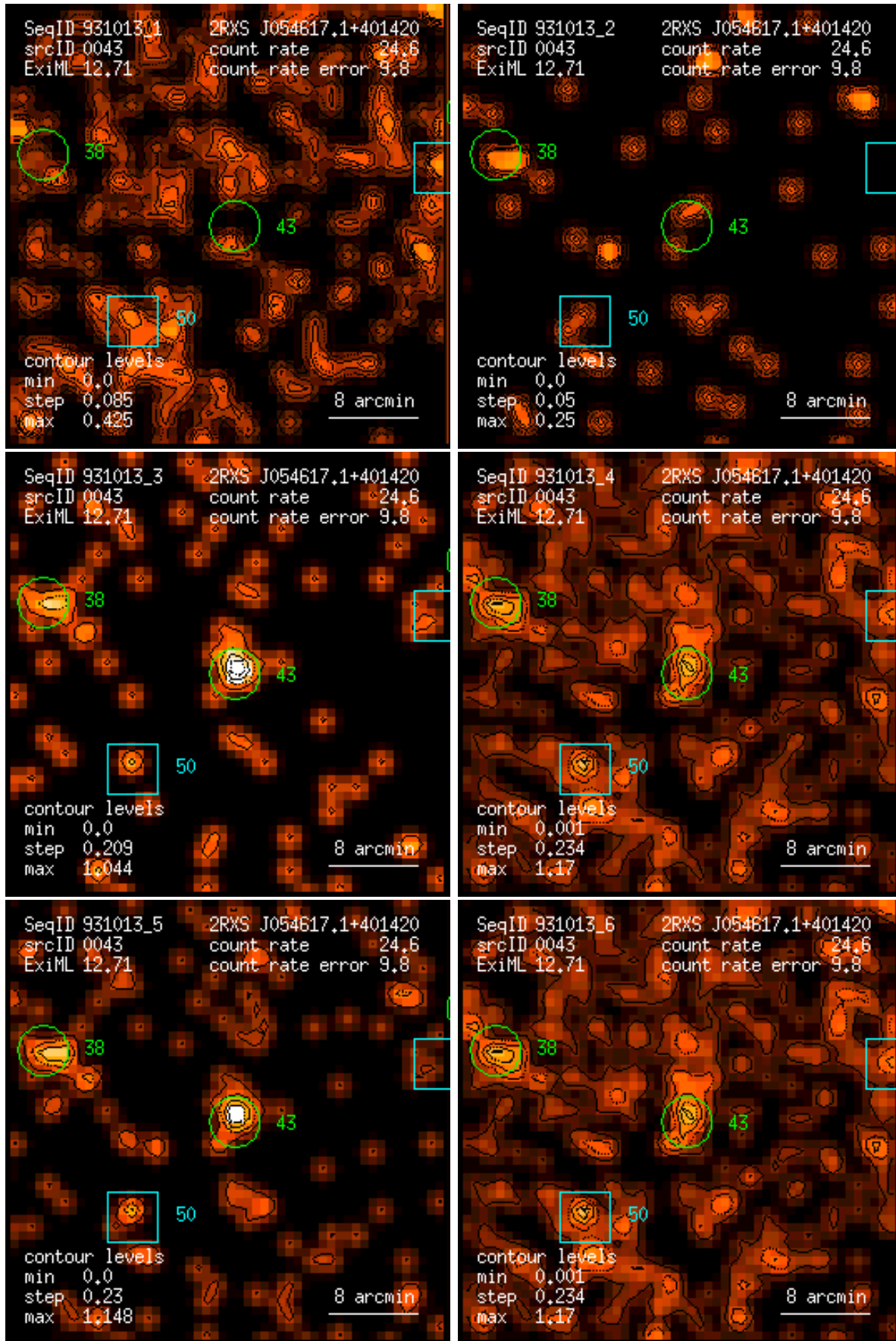
Figure 43: RASS 931013: detection 0043: band rate images, Gaussian filter: (1) PSPC channels 11 – 41, (2) 52 – 90, (3) 91 – 201, (4) 11 – 235, (5) 52 – 201, (6) 11 – 201. Broad band rates in counts/ks. Band rate contour levels in counts/ks/arcmin 2 .
