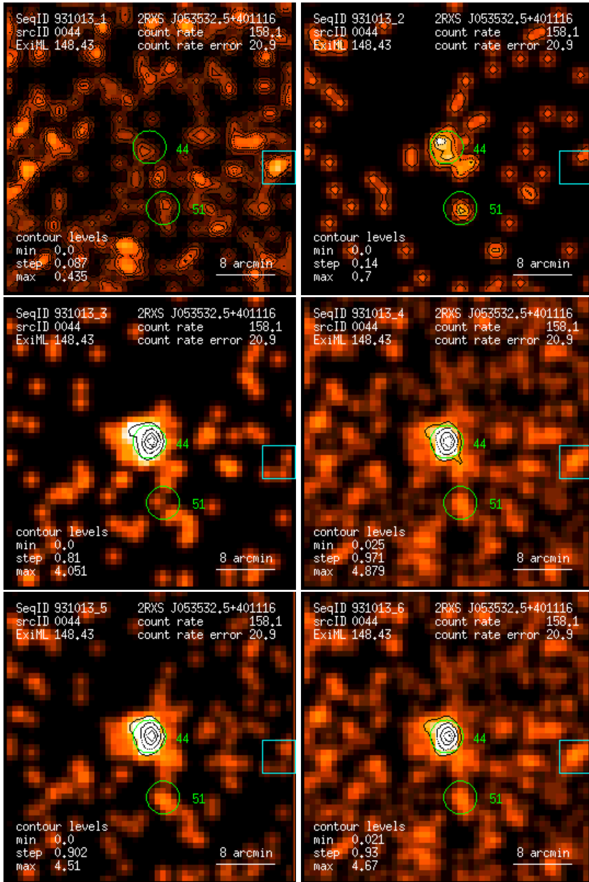
Figure 44: RASS 931013: detection 0044: band rate images, Gaussian filter: (1) PSPC channels 11 – 41, (2) 52 – 90, (3) 91 – 201, (4) 11 – 235, (5) 52 – 201, (6) 11 – 201. Broad band rates in counts/ks. Band rate contour levels in counts/ks/arcmin 2 .
