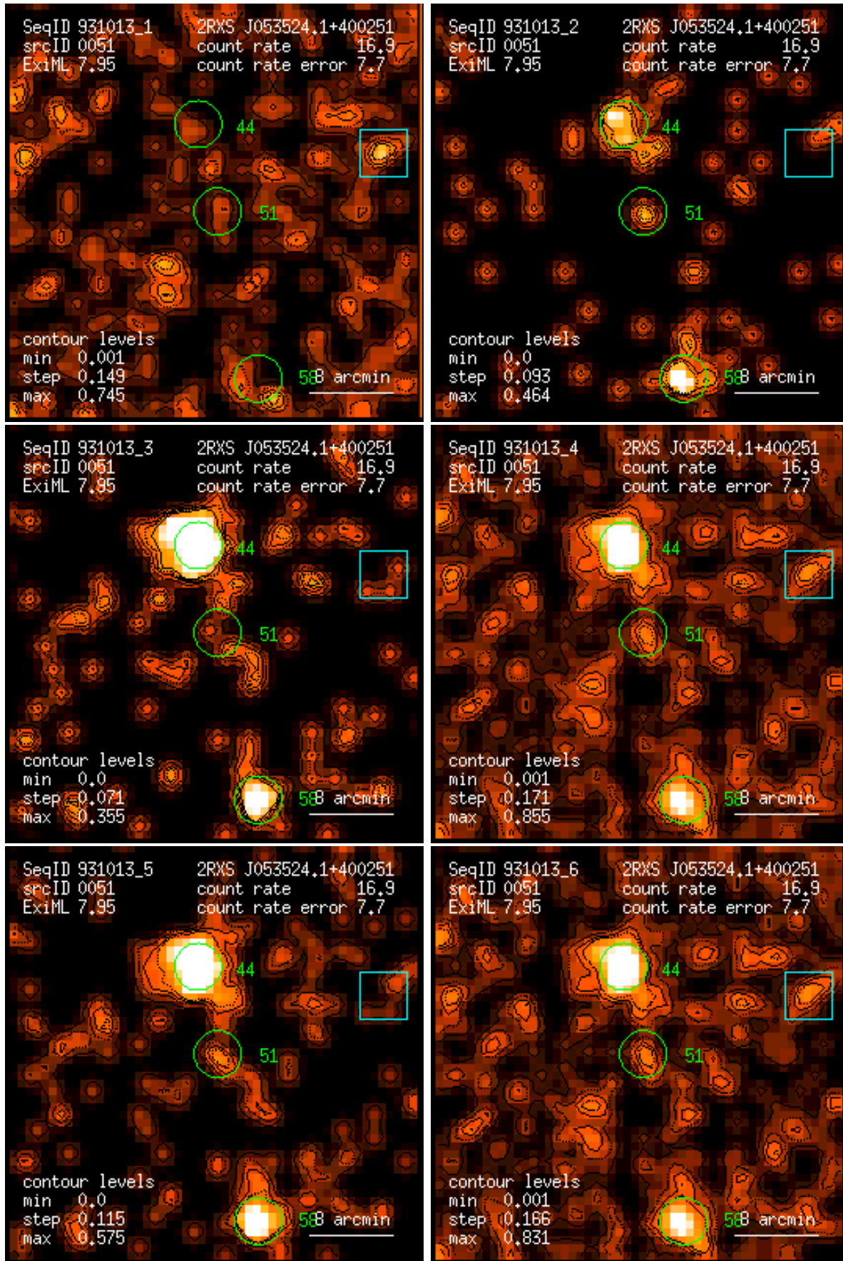
Figure 51: RASS 931013: detection 0051: band rate images, Gaussian filter: (1) PSPC channels 11 – 41, (2) 52 – 90, (3) 91 – 201, (4) 11 – 235, (5) 52 – 201, (6) 11 – 201. Broad band rates in counts/ks. Band rate contour levels in counts/ks/arcmin 2 .
