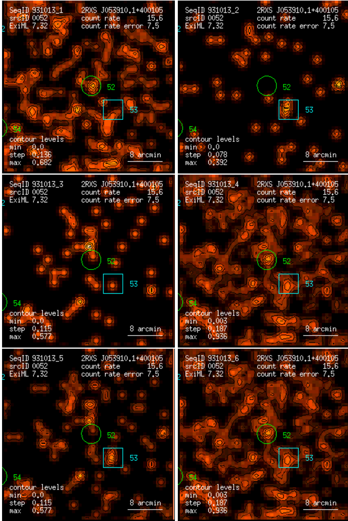
Figure 52: RASS 931013: detection 0052: band rate images, Gaussian filter: (1) PSPC channels 11 – 41, (2) 52 – 90, (3) 91 – 201, (4) 11 – 235, (5) 52 – 201, (6) 11 – 201. Broad band rates in counts/ks. Band rate contour levels in counts/ks/arcmin 2 .
