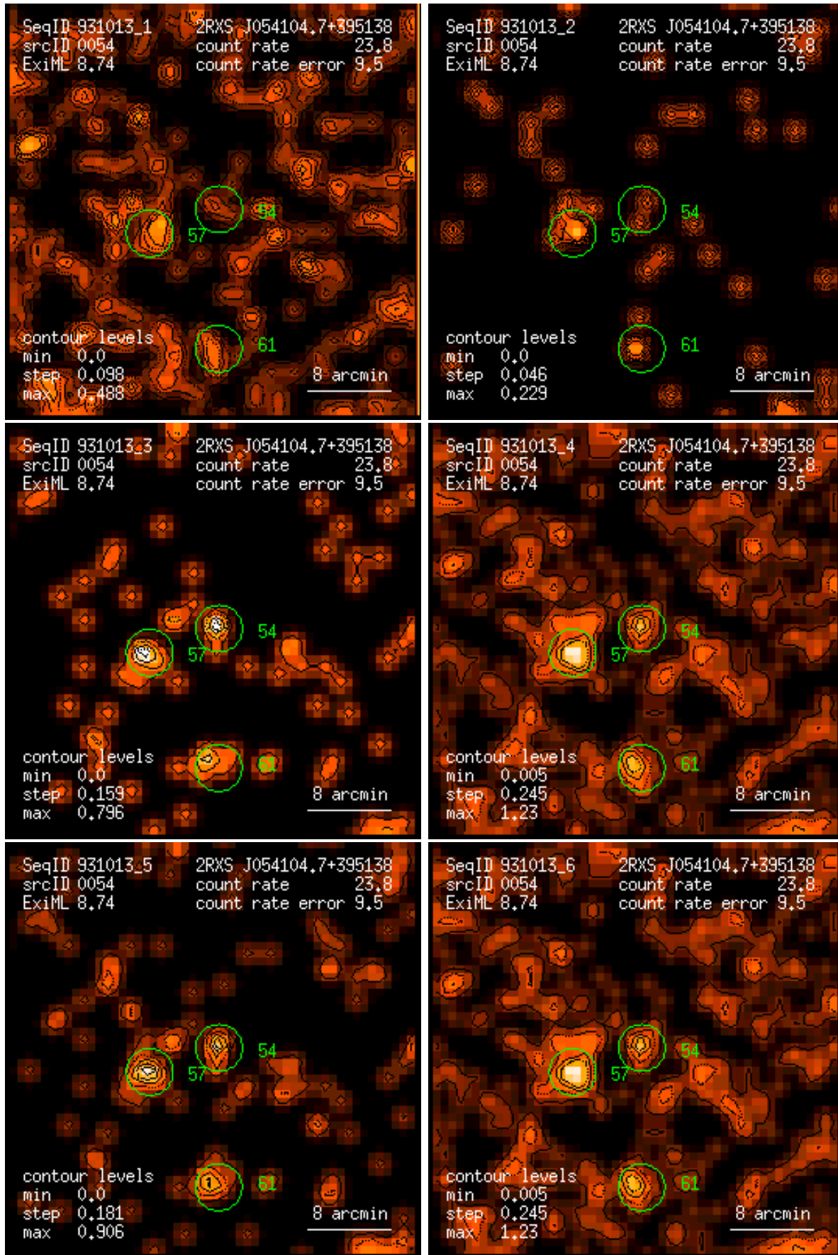
Figure 54: RASS 931013: detection 0054: band rate images, Gaussian filter: (1) PSPC channels 11 – 41, (2) 52 – 90, (3) 91 – 201, (4) 11 – 235, (5) 52 – 201, (6) 11 – 201. Broad band rates in counts/ks. Band rate contour levels in counts/ks/arcmin 2 .
