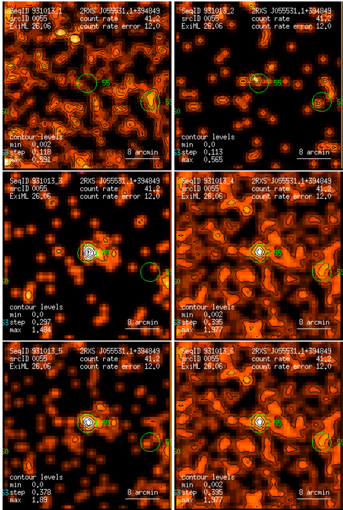
Figure 55: RASS 931013: detection 0055: band rate images, Gaussian filter: (1) PSPC channels 11 – 41, (2) 52 – 90, (3) 91 – 201, (4) 11 – 235, (5) 52 – 201, (6) 11 – 201. Broad band rates in counts/ks. Band rate contour levels in counts/ks/arcmin 2 .
