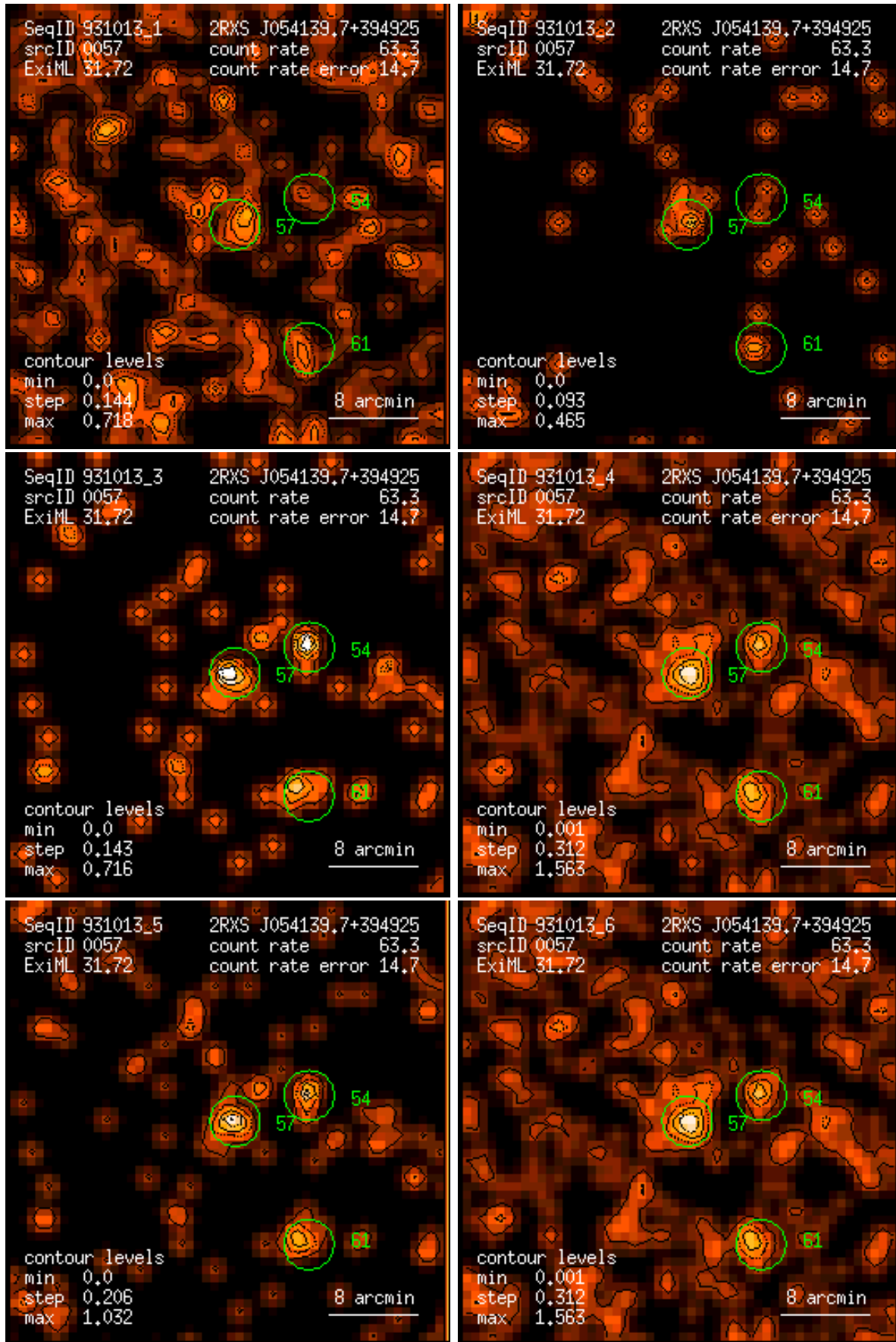
Figure 57: RASS 931013: detection 0057: band rate images, Gaussian filter: (1) PSPC channels 11 – 41, (2) 52 – 90, (3) 91 – 201, (4) 11 – 235, (5) 52 – 201, (6) 11 – 201. Broad band rates in counts/ks. Band rate contour levels in counts/ks/arcmin 2 .
