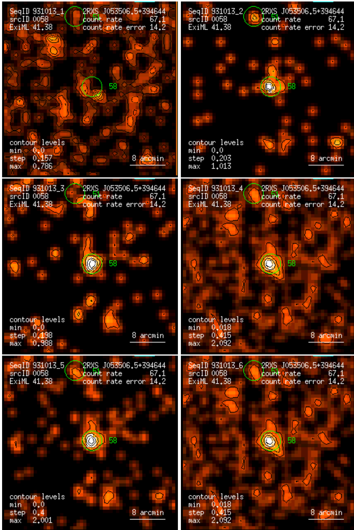
Figure 58: RASS 931013: detection 0058: band rate images, Gaussian filter: (1) PSPC channels 11 – 41, (2) 52 – 90, (3) 91 – 201, (4) 11 – 235, (5) 52 – 201, (6) 11 – 201. Broad band rates in counts/ks. Band rate contour levels in counts/ks/arcmin 2 .
