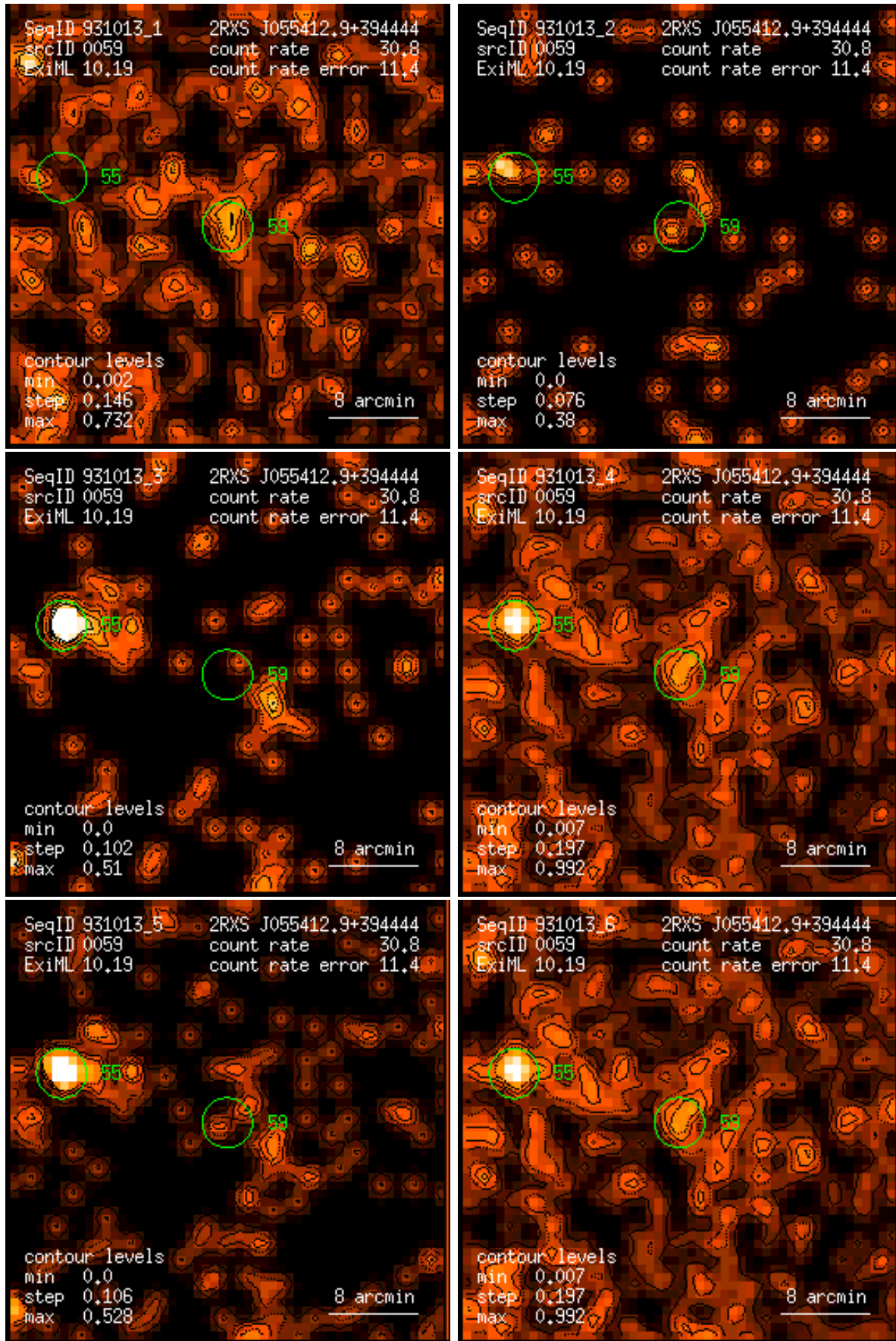
Figure 59: RASS 931013: detection 0059: band rate images, Gaussian filter: (1) PSPC channels 11 – 41, (2) 52 – 90, (3) 91 – 201, (4) 11 – 235, (5) 52 – 201, (6) 11 – 201. Broad band rates in counts/ks. Band rate contour levels in counts/ks/arcmin 2 .
