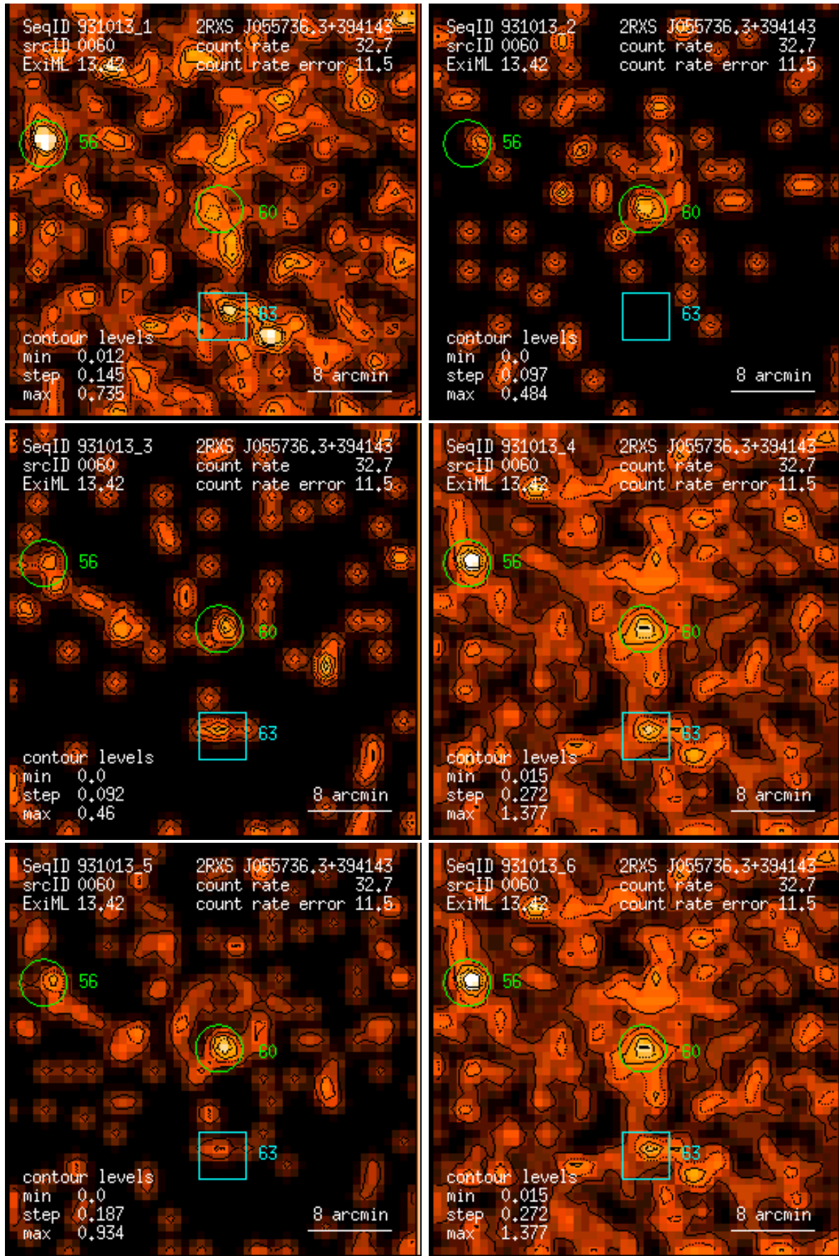
Figure 60: RASS 931013: detection 0060: band rate images, Gaussian filter: (1) PSPC channels 11 – 41, (2) 52 – 90, (3) 91 – 201, (4) 11 – 235, (5) 52 – 201, (6) 11 – 201. Broad band rates in counts/ks. Band rate contour levels in counts/ks/arcmin 2 .
