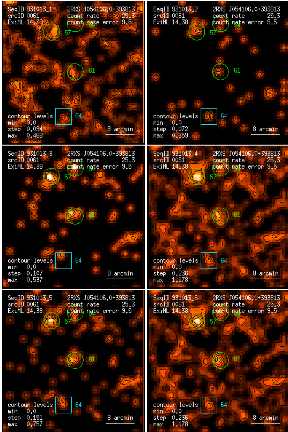
Figure 61: RASS 931013: detection 0061: band rate images, Gaussian filter: (1) PSPC channels 11 – 41, (2) 52 – 90, (3) 91 – 201, (4) 11 – 235, (5) 52 – 201, (6) 11 – 201. Broad band rates in counts/ks. Band rate contour levels in counts/ks/arcmin 2 .
