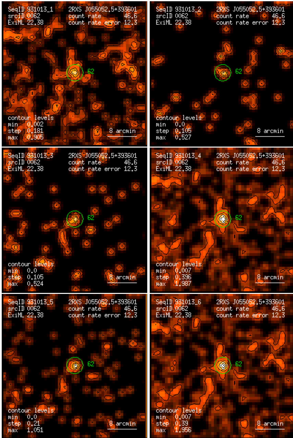
Figure 62: RASS 931013: detection 0062: band rate images, Gaussian filter: (1) PSPC channels 11 – 41, (2) 52 – 90, (3) 91 – 201, (4) 11 – 235, (5) 52 – 201, (6) 11 – 201. Broad band rates in counts/ks. Band rate contour levels in counts/ks/arcmin 2 .
