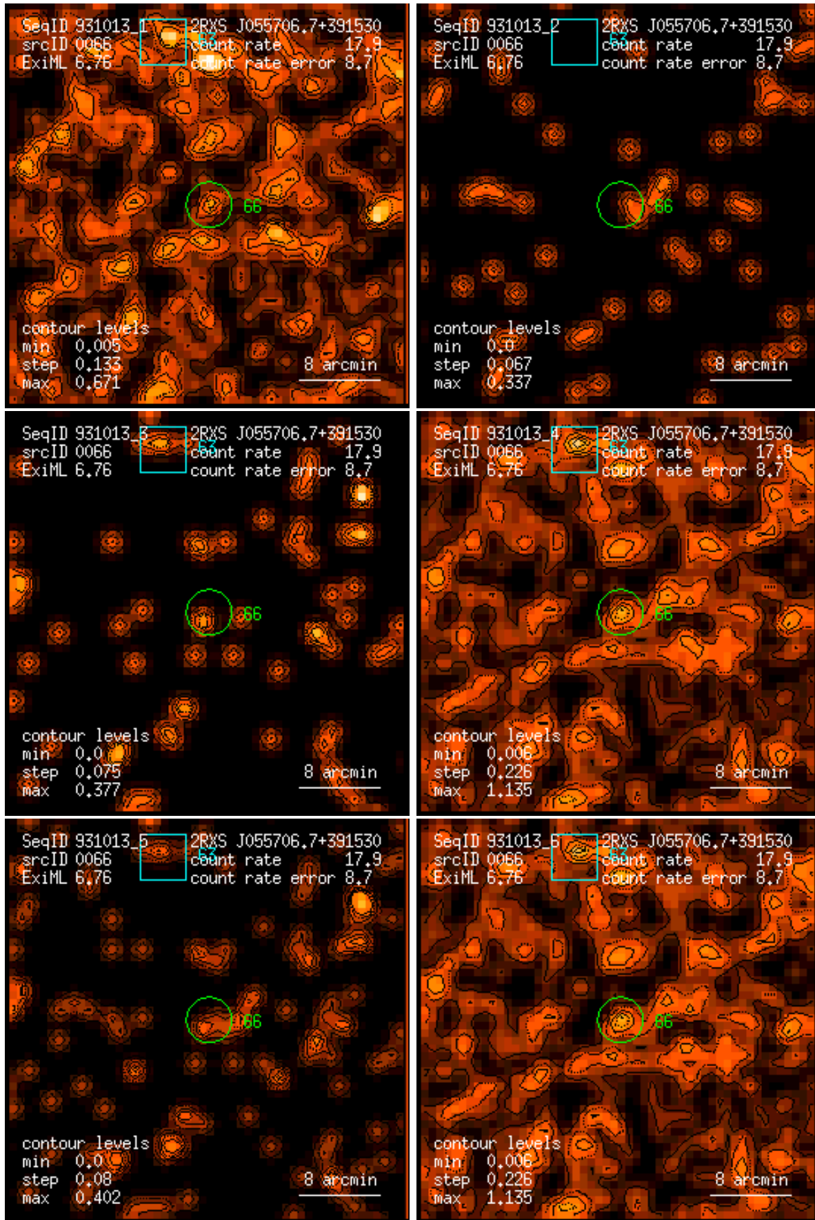
Figure 66: RASS 931013: detection 0066: band rate images, Gaussian filter: (1) PSPC channels 11 – 41, (2) 52 – 90, (3) 91 – 201, (4) 11 – 235, (5) 52 – 201, (6) 11 – 201. Broad band rates in counts/ks. Band rate contour levels in counts/ks/arcmin 2 .
