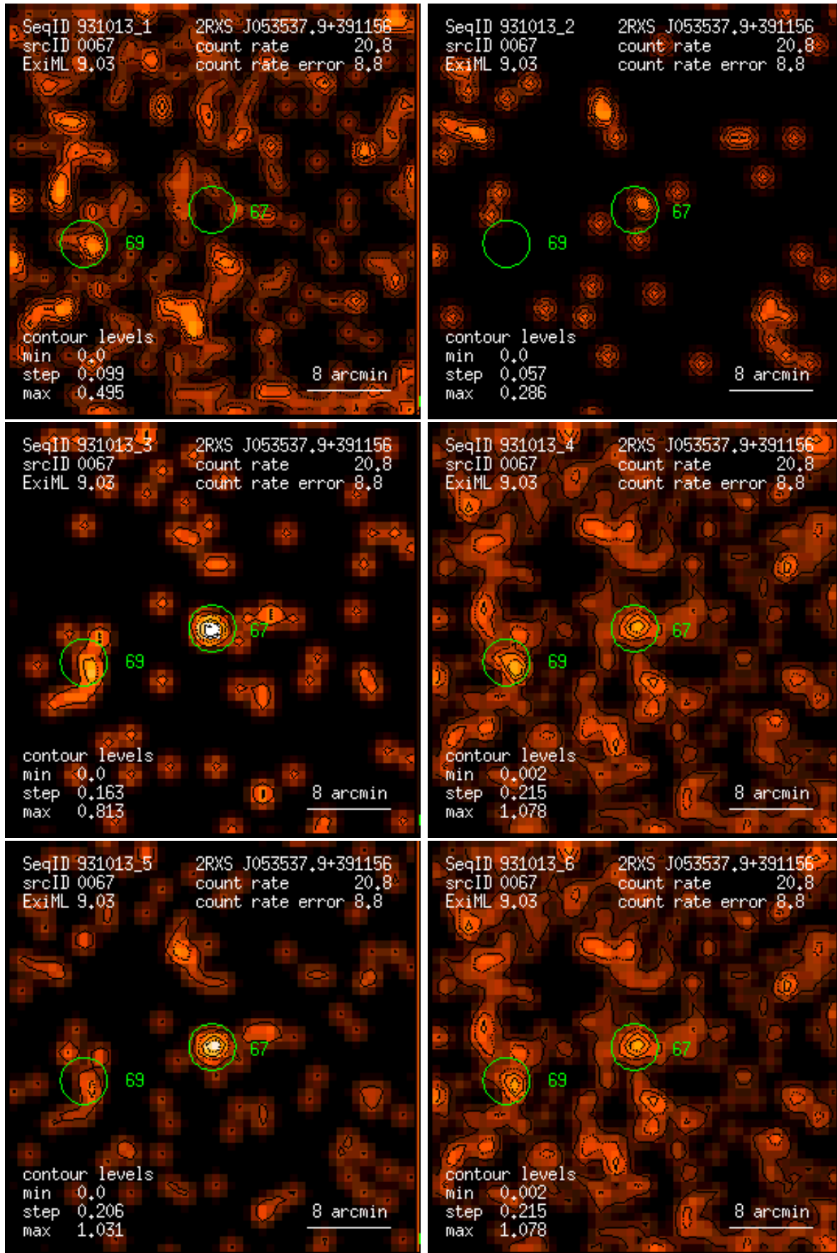
Figure 67: RASS 931013: detection 0067: band rate images, Gaussian filter: (1) PSPC channels 11 – 41, (2) 52 – 90, (3) 91 – 201, (4) 11 – 235, (5) 52 – 201, (6) 11 – 201. Broad band rates in counts/ks. Band rate contour levels in counts/ks/arcmin 2 .
