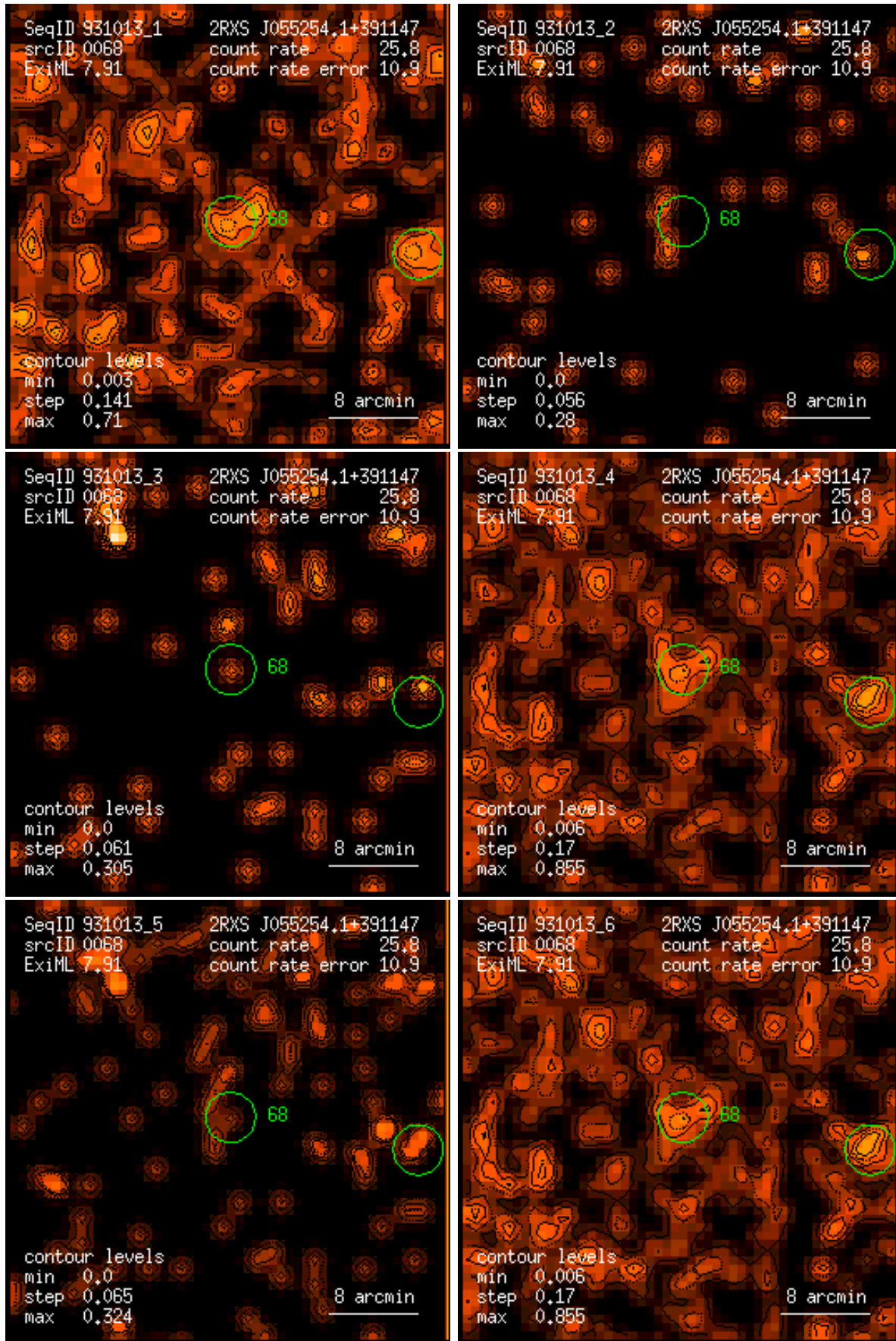
Figure 68: RASS 931013: detection 0068: band rate images, Gaussian filter: (1) PSPC channels 11 – 41, (2) 52 – 90, (3) 91 – 201, (4) 11 – 235, (5) 52 – 201, (6) 11 – 201. Broad band rates in counts/ks. Band rate contour levels in counts/ks/arcmin 2 .
