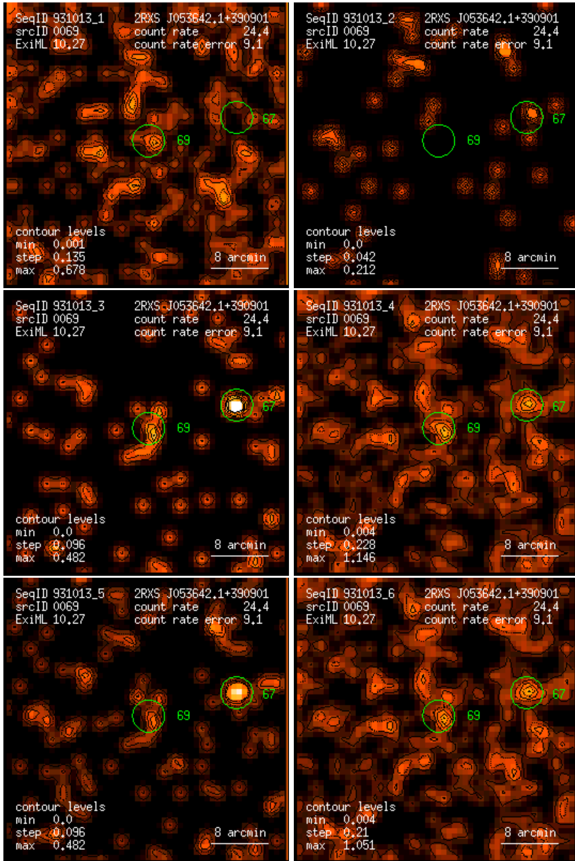
Figure 69: RASS 931013: detection 0069: band rate images, Gaussian filter: (1) PSPC channels 11 – 41, (2) 52 – 90, (3) 91 – 201, (4) 11 – 235, (5) 52 – 201, (6) 11 – 201. Broad band rates in counts/ks. Band rate contour levels in counts/ks/arcmin 2 .
