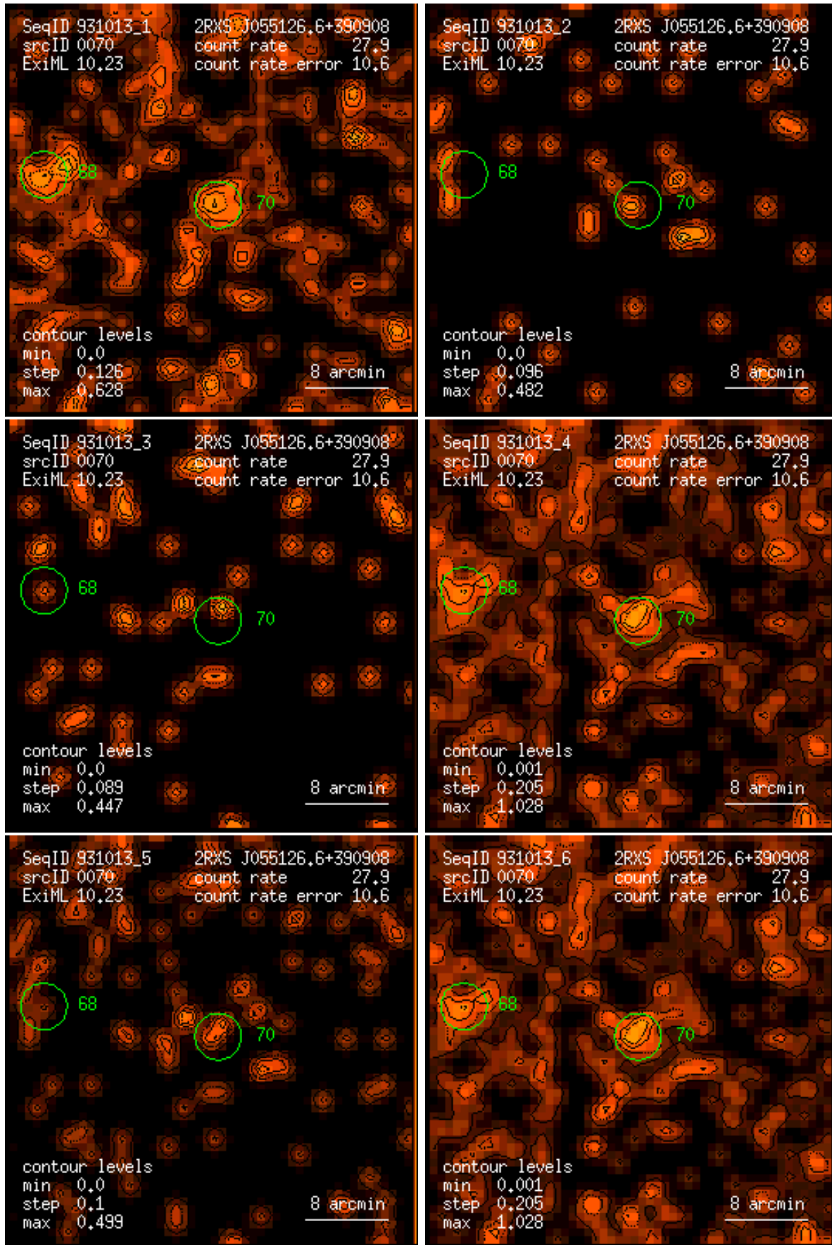
Figure 70: RASS 931013: detection 0070: band rate images, Gaussian filter: (1) PSPC channels 11 – 41, (2) 52 – 90, (3) 91 – 201, (4) 11 – 235, (5) 52 – 201, (6) 11 – 201. Broad band rates in counts/ks. Band rate contour levels in counts/ks/arcmin 2 .
