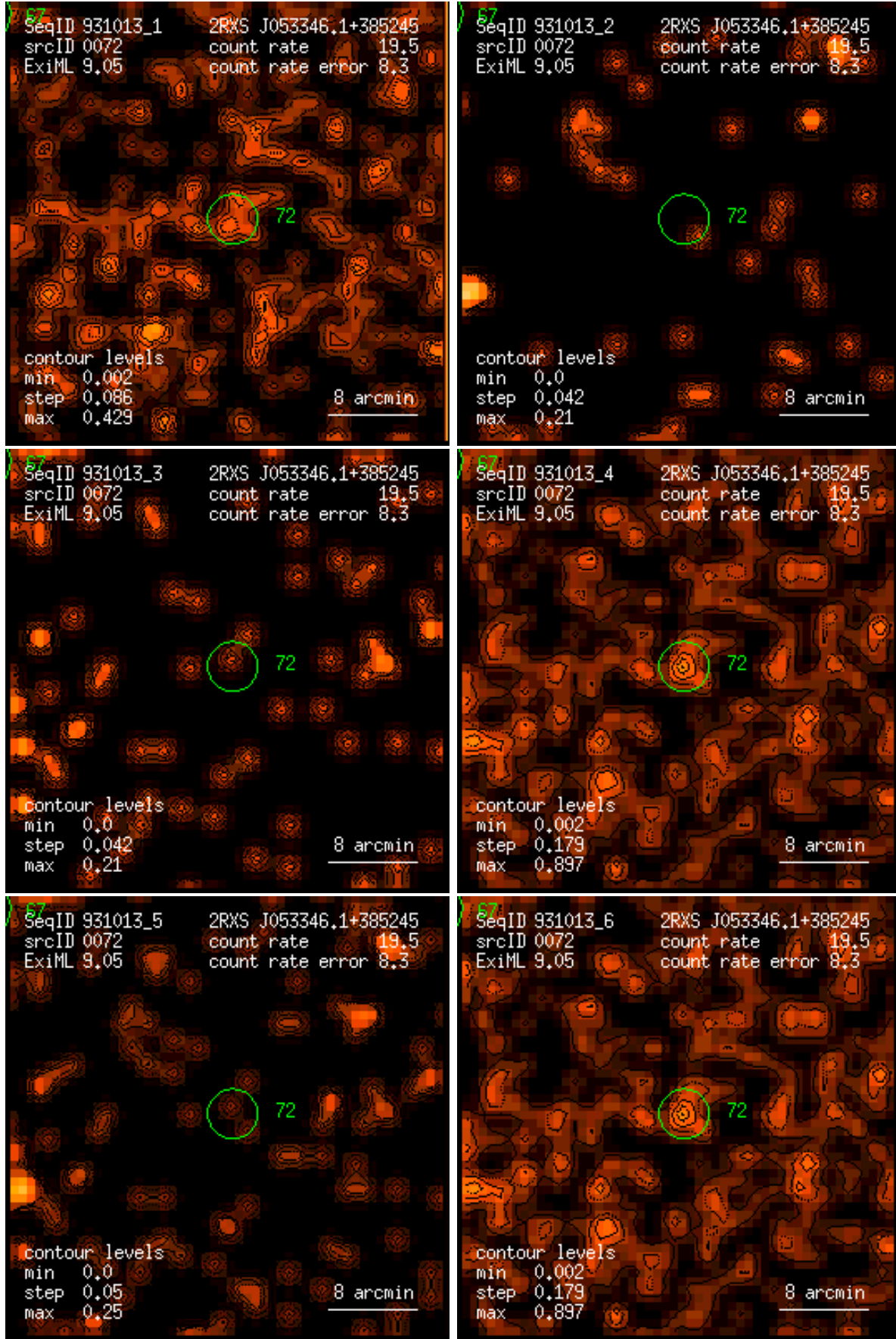
Figure 72: RASS 931013: detection 0072: band rate images, Gaussian filter: (1) PSPC channels 11 – 41, (2) 52 – 90, (3) 91 – 201, (4) 11 – 235, (5) 52 – 201, (6) 11 – 201. Broad band rates in counts/ks. Band rate contour levels in counts/ks/arcmin 2 .
