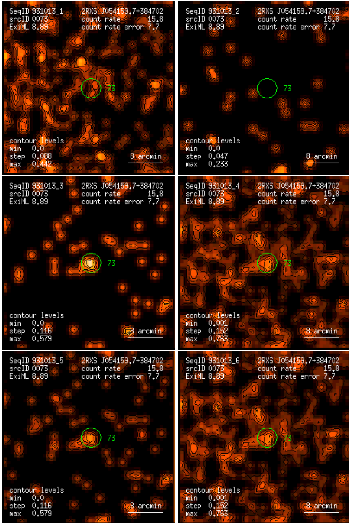
Figure 73: RASS 931013: detection 0073: band rate images, Gaussian filter: (1) PSPC channels 11 – 41, (2) 52 – 90, (3) 91 – 201, (4) 11 – 235, (5) 52 – 201, (6) 11 – 201. Broad band rates in counts/ks. Band rate contour levels in counts/ks/arcmin 2 .
