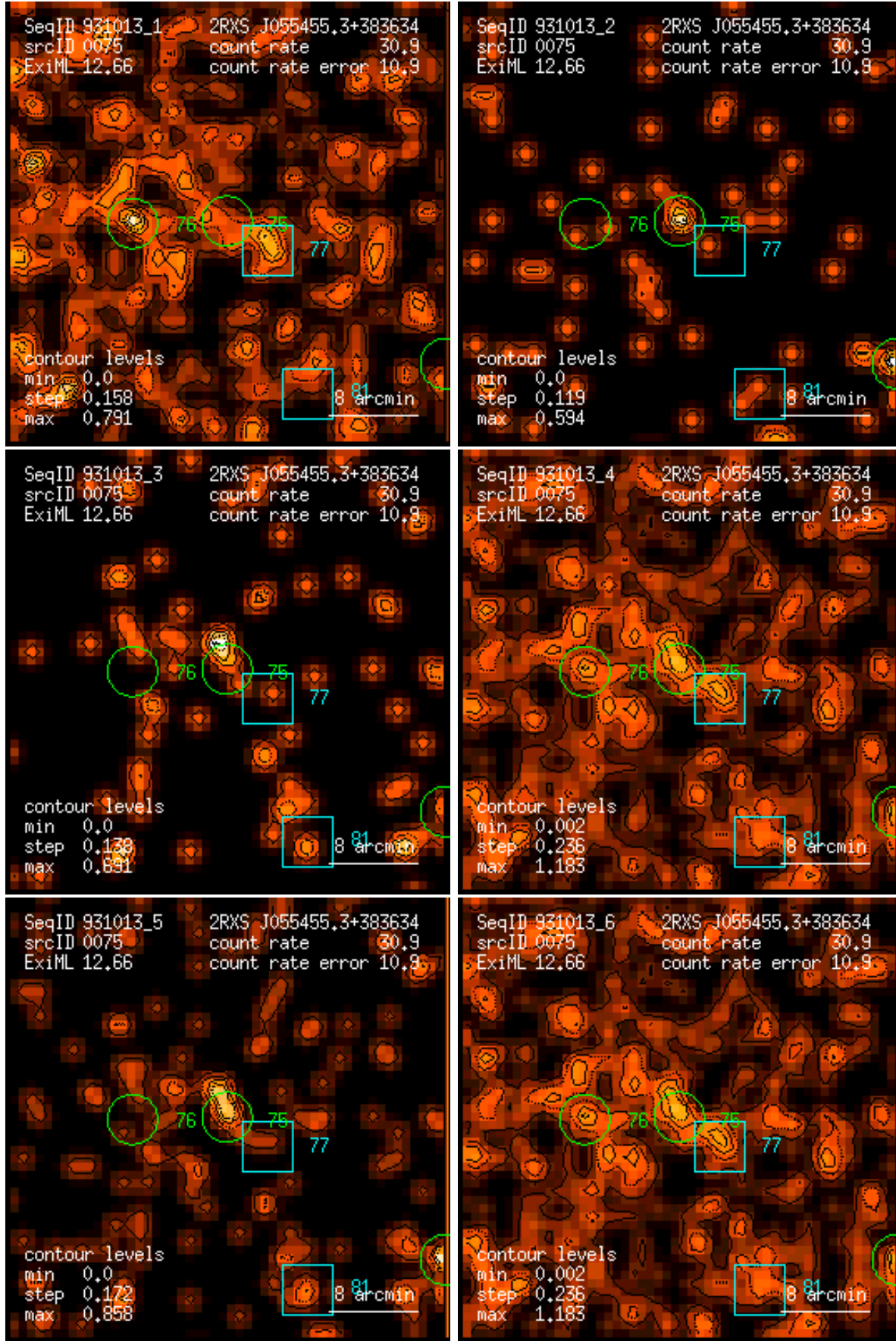
Figure 75: RASS 931013: detection 0075: band rate images, Gaussian filter: (1) PSPC channels 11 – 41, (2) 52 – 90, (3) 91 – 201, (4) 11 – 235, (5) 52 – 201, (6) 11 – 201. Broad band rates in counts/ks. Band rate contour levels in counts/ks/arcmin 2 .
