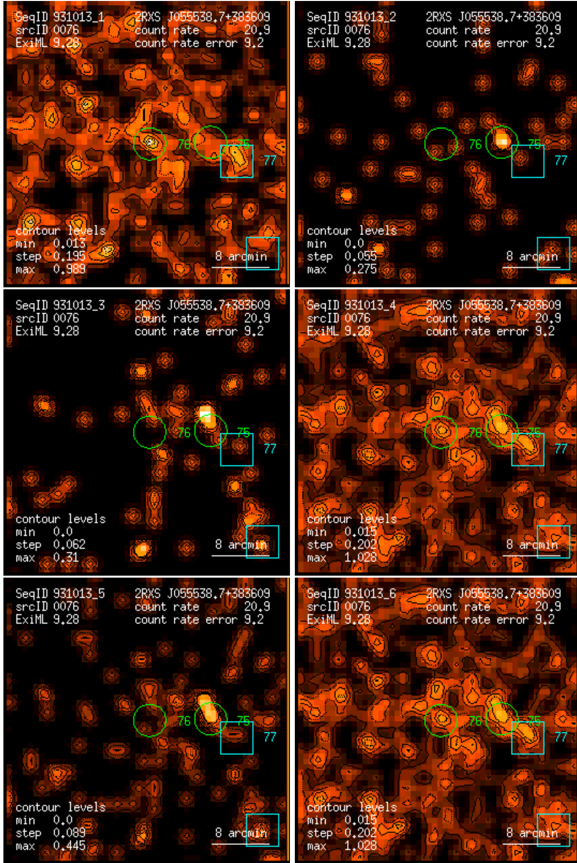
Figure 76: RASS 931013: detection 0076: band rate images, Gaussian filter: (1) PSPC channels 11 – 41, (2) 52 – 90, (3) 91 – 201, (4) 11 – 235, (5) 52 – 201, (6) 11 – 201. Broad band rates in counts/ks. Band rate contour levels in counts/ks/arcmin 2 .
