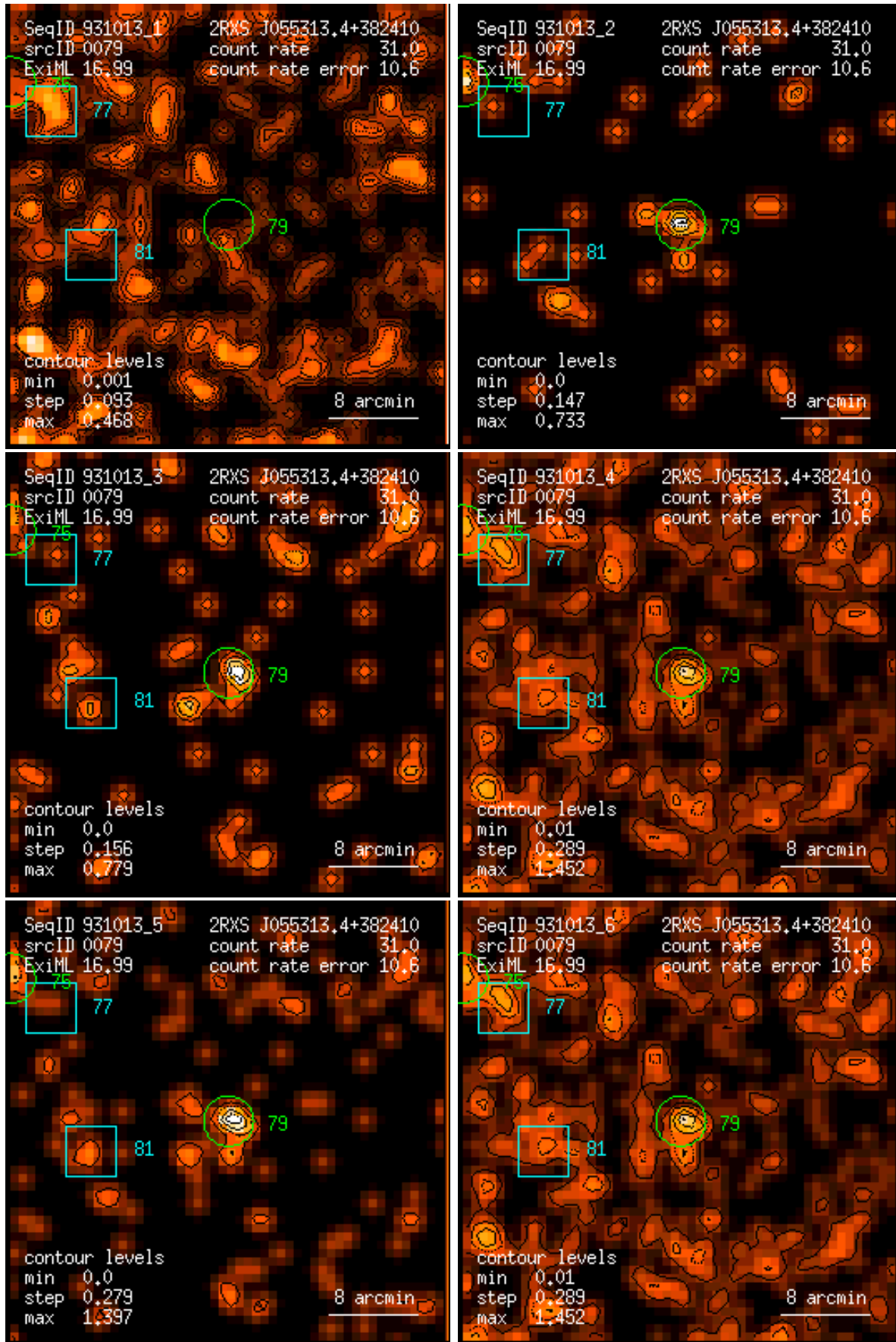
Figure 79: RASS 931013: detection 0079: band rate images, Gaussian filter: (1) PSPC channels 11 – 41, (2) 52 – 90, (3) 91 – 201, (4) 11 – 235, (5) 52 – 201, (6) 11 – 201. Broad band rates in counts/ks. Band rate contour levels in counts/ks/arcmin 2 .
