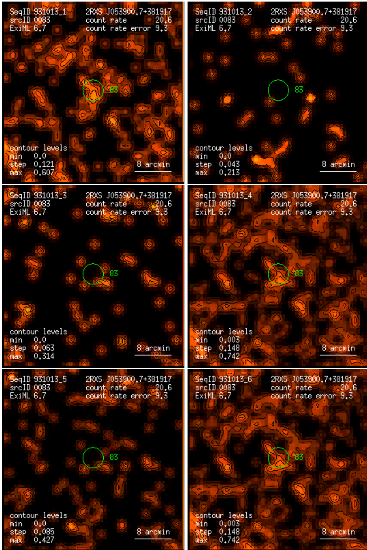
Figure 83: RASS 931013: detection 0083: band rate images, Gaussian filter: (1) PSPC channels 11 – 41, (2) 52 – 90, (3) 91 – 201, (4) 11 – 235, (5) 52 – 201, (6) 11 – 201. Broad band rates in counts/ks. Band rate contour levels in counts/ks/arcmin 2 .
