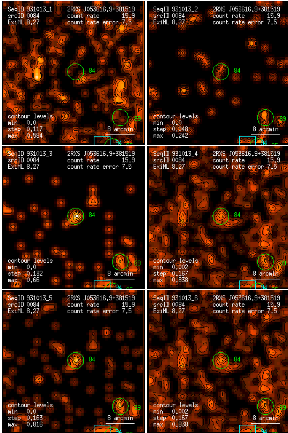
Figure 84: RASS 931013: detection 0084: band rate images, Gaussian filter: (1) PSPC channels 11 – 41, (2) 52 – 90, (3) 91 – 201, (4) 11 – 235, (5) 52 – 201, (6) 11 – 201. Broad band rates in counts/ks. Band rate contour levels in counts/ks/arcmin 2 .
