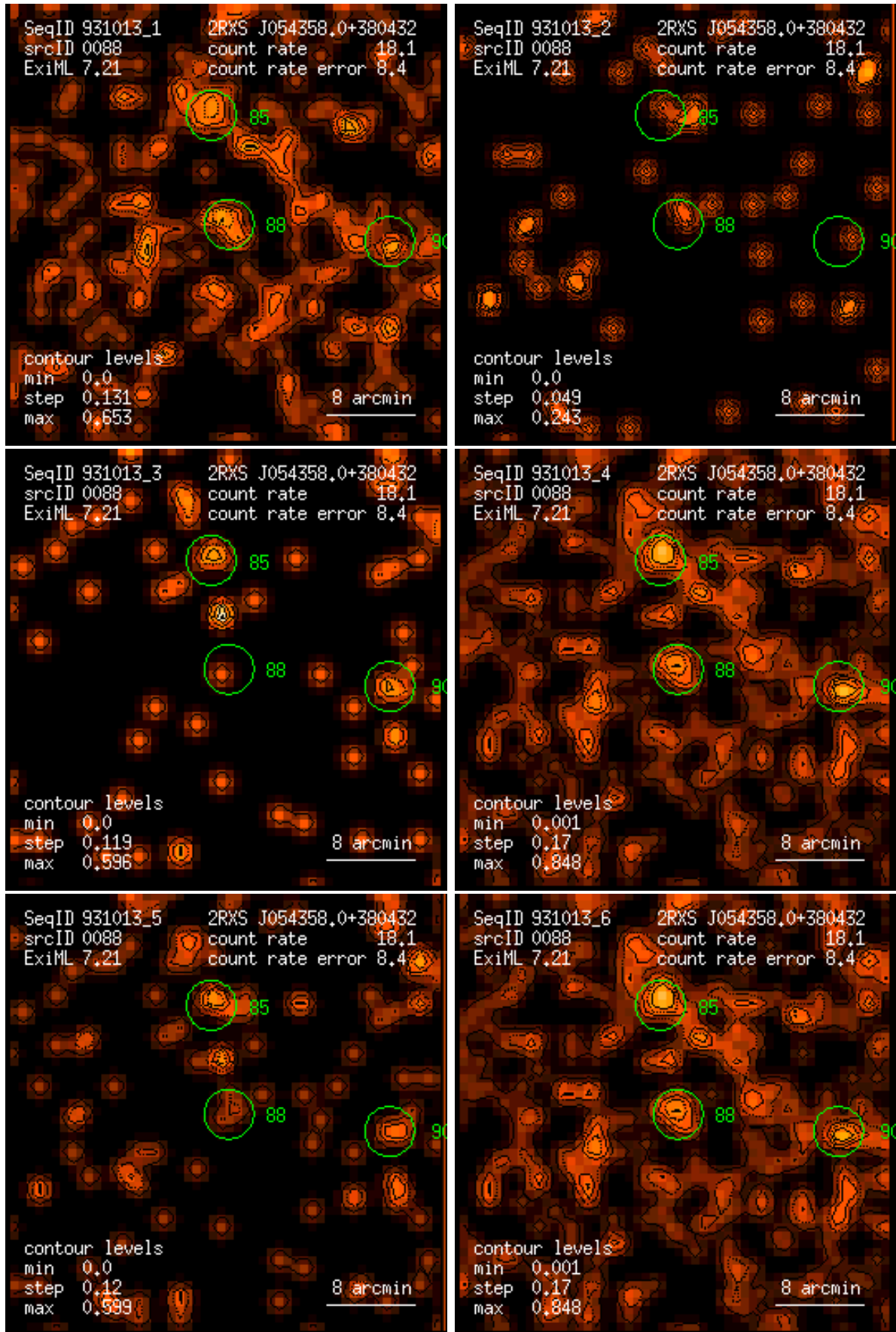
Figure 88: RASS 931013: detection 0088: band rate images, Gaussian filter: (1) PSPC channels 11 – 41, (2) 52 – 90, (3) 91 – 201, (4) 11 – 235, (5) 52 – 201, (6) 11 – 201. Broad band rates in counts/ks. Band rate contour levels in counts/ks/arcmin 2 .
