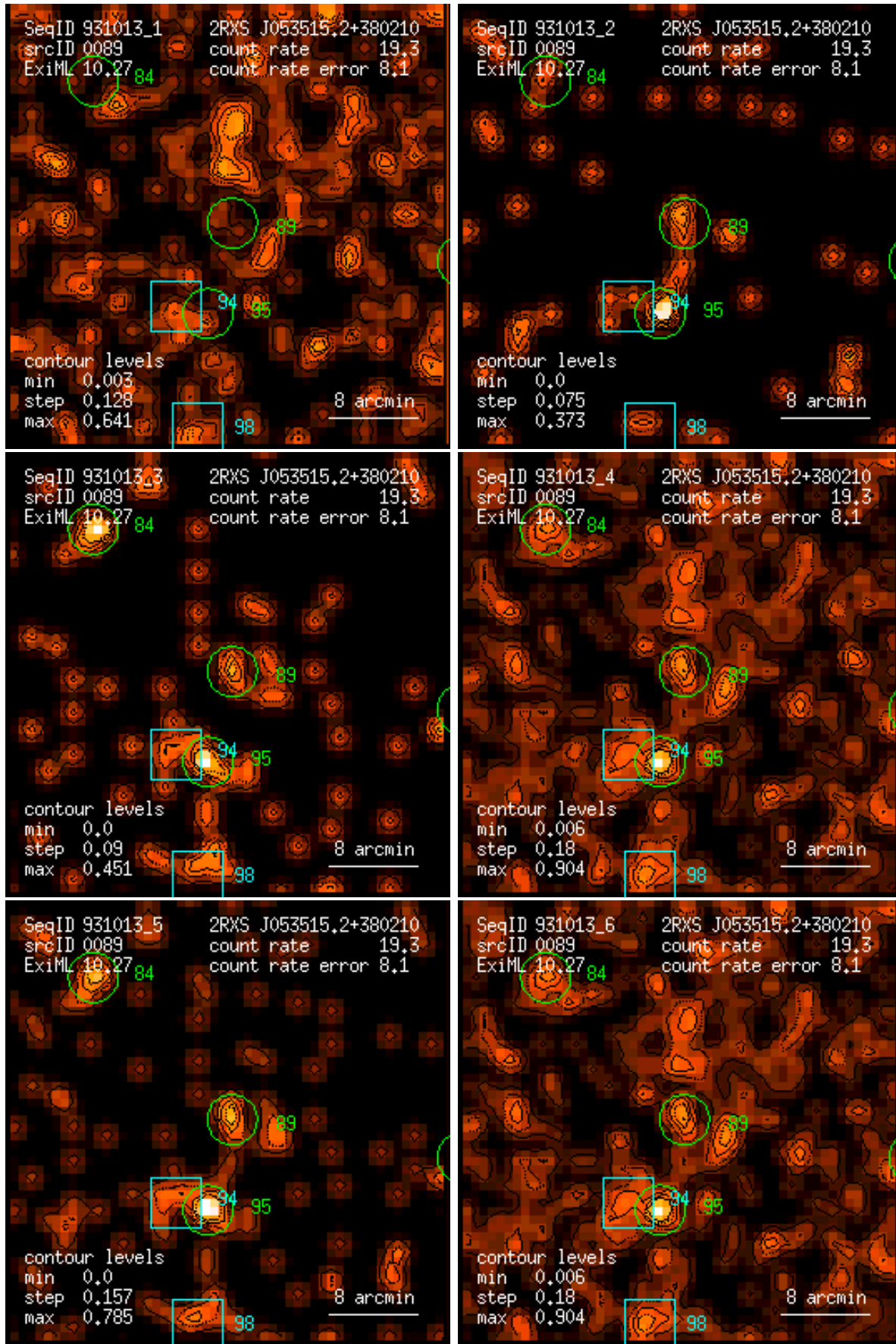
Figure 89: RASS 931013: detection 0089: band rate images, Gaussian filter: (1) PSPC channels 11 – 41, (2) 52 – 90, (3) 91 – 201, (4) 11 – 235, (5) 52 – 201, (6) 11 – 201. Broad band rates in counts/ks. Band rate contour levels in counts/ks/arcmin 2 .
