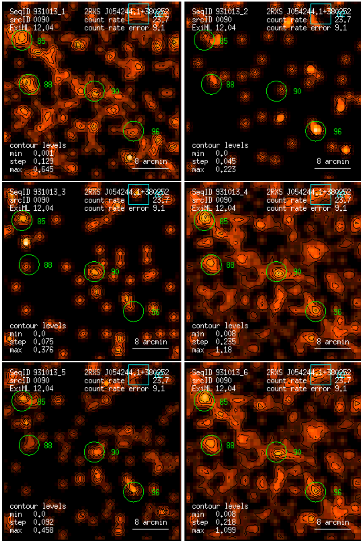
Figure 90: RASS 931013: detection 0090: band rate images, Gaussian filter: (1) PSPC channels 11 – 41, (2) 52 – 90, (3) 91 – 201, (4) 11 – 235, (5) 52 – 201, (6) 11 – 201. Broad band rates in counts/ks. Band rate contour levels in counts/ks/arcmin 2 .
