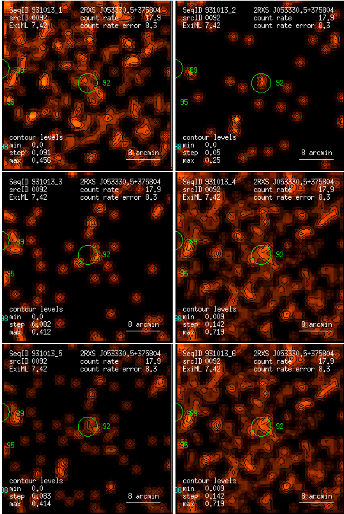
Figure 92: RASS 931013: detection 0092: band rate images, Gaussian filter: (1) PSPC channels 11 – 41, (2) 52 – 90, (3) 91 – 201, (4) 11 – 235, (5) 52 – 201, (6) 11 – 201. Broad band rates in counts/ks. Band rate contour levels in counts/ks/arcmin 2 .
