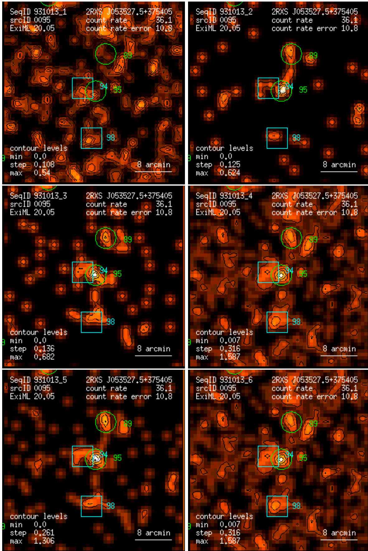
Figure 95: RASS 931013: detection 0095: band rate images, Gaussian filter: (1) PSPC channels 11 – 41, (2) 52 – 90, (3) 91 – 201, (4) 11 – 235, (5) 52 – 201, (6) 11 – 201. Broad band rates in counts/ks. Band rate contour levels in counts/ks/arcmin 2 .
