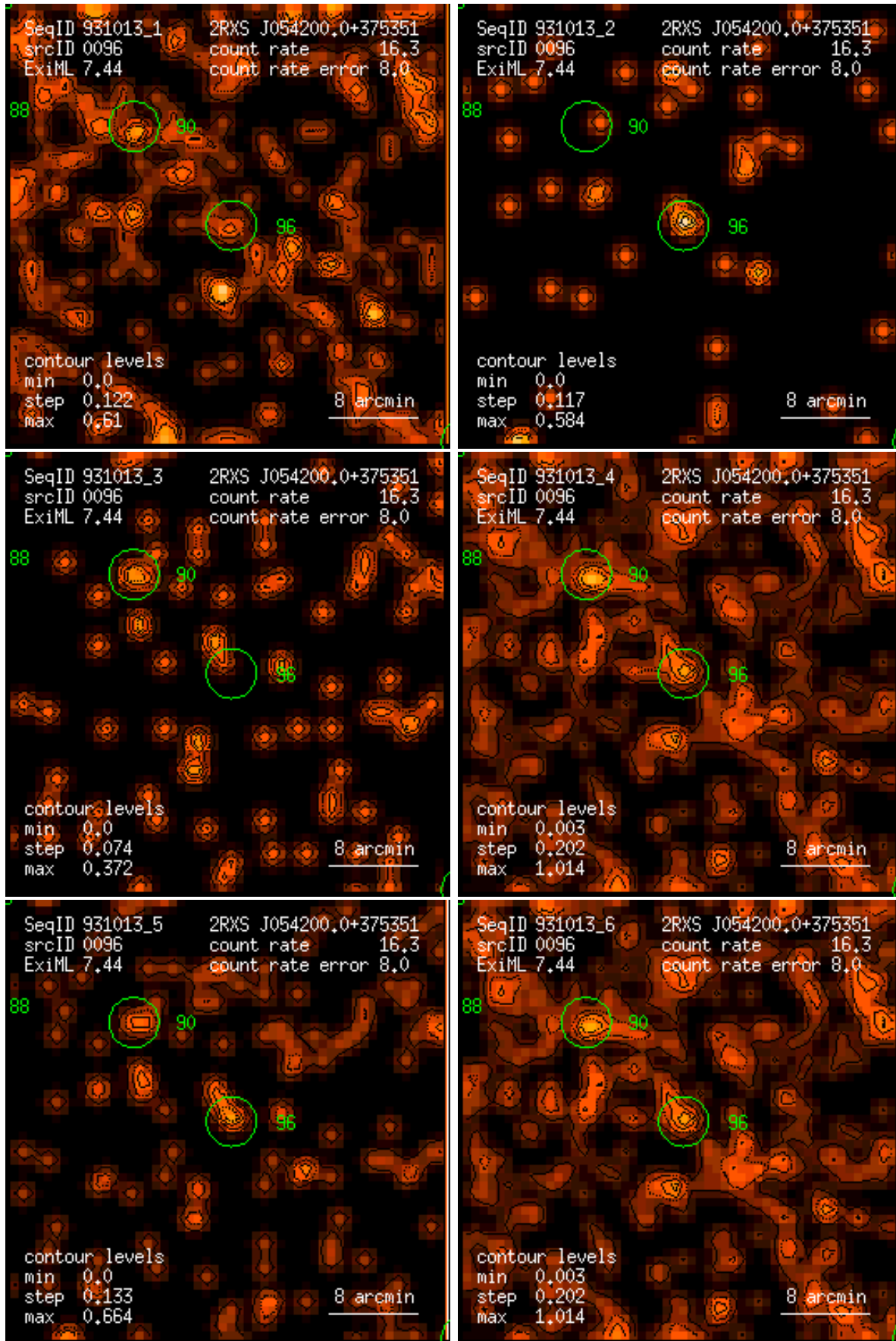
Figure 96: RASS 931013: detection 0096: band rate images, Gaussian filter: (1) PSPC channels 11 – 41, (2) 52 – 90, (3) 91 – 201, (4) 11 – 235, (5) 52 – 201, (6) 11 – 201. Broad band rates in counts/ks. Band rate contour levels in counts/ks/arcmin 2 .
