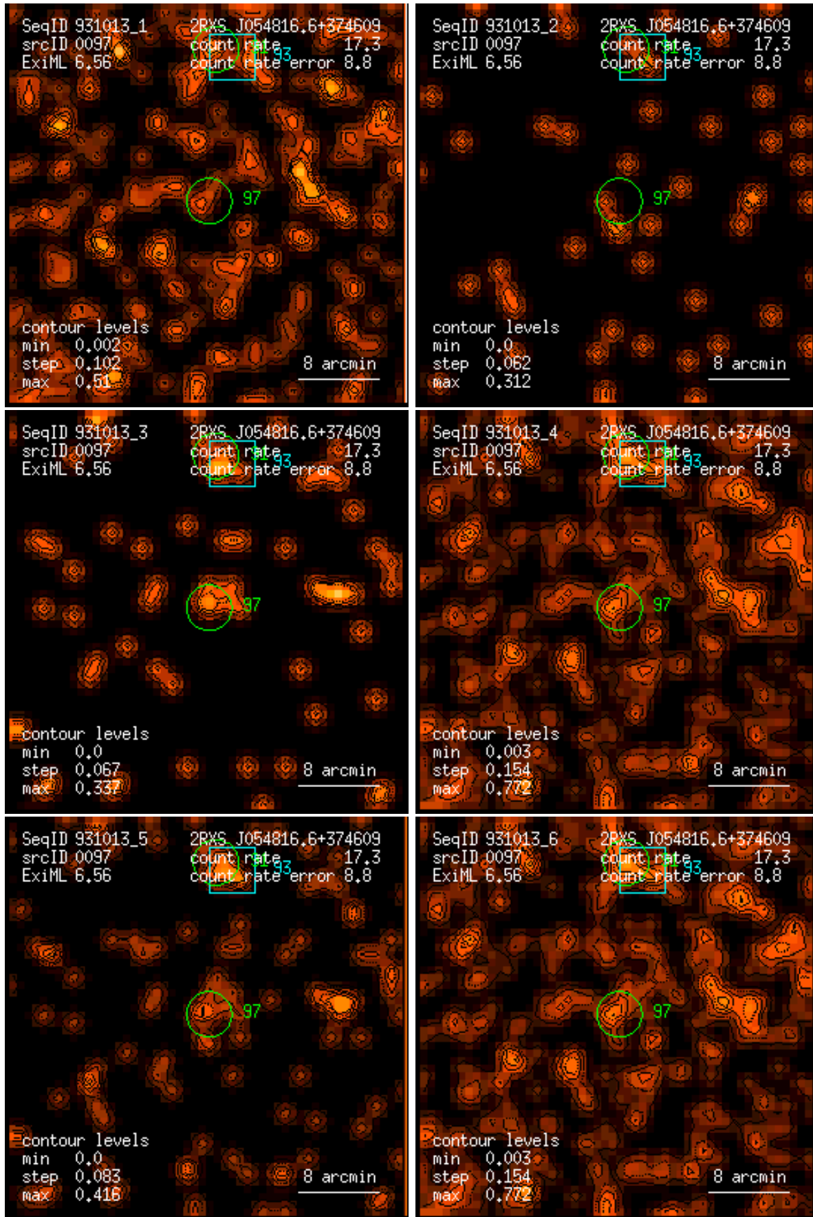
Figure 97: RASS 931013: detection 0097: band rate images, Gaussian filter: (1) PSPC channels 11 – 41, (2) 52 – 90, (3) 91 – 201, (4) 11 – 235, (5) 52 – 201, (6) 11 – 201. Broad band rates in counts/ks. Band rate contour levels in counts/ks/arcmin 2 .
