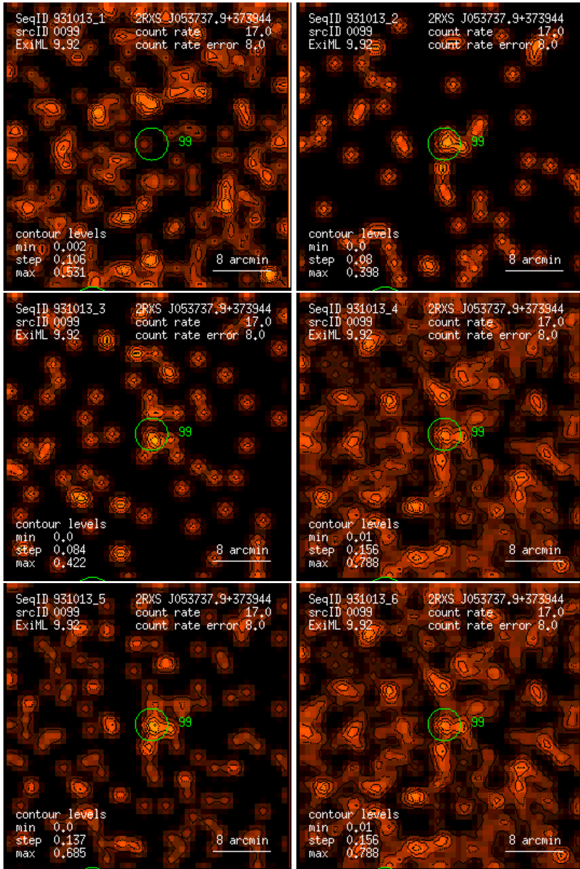
Figure 99: RASS 931013: detection 0099: band rate images, Gaussian filter: (1) PSPC channels 11 – 41, (2) 52 – 90, (3) 91 – 201, (4) 11 – 235, (5) 52 – 201, (6) 11 – 201. Broad band rates in counts/ks. Band rate contour levels in counts/ks/arcmin 2 .
