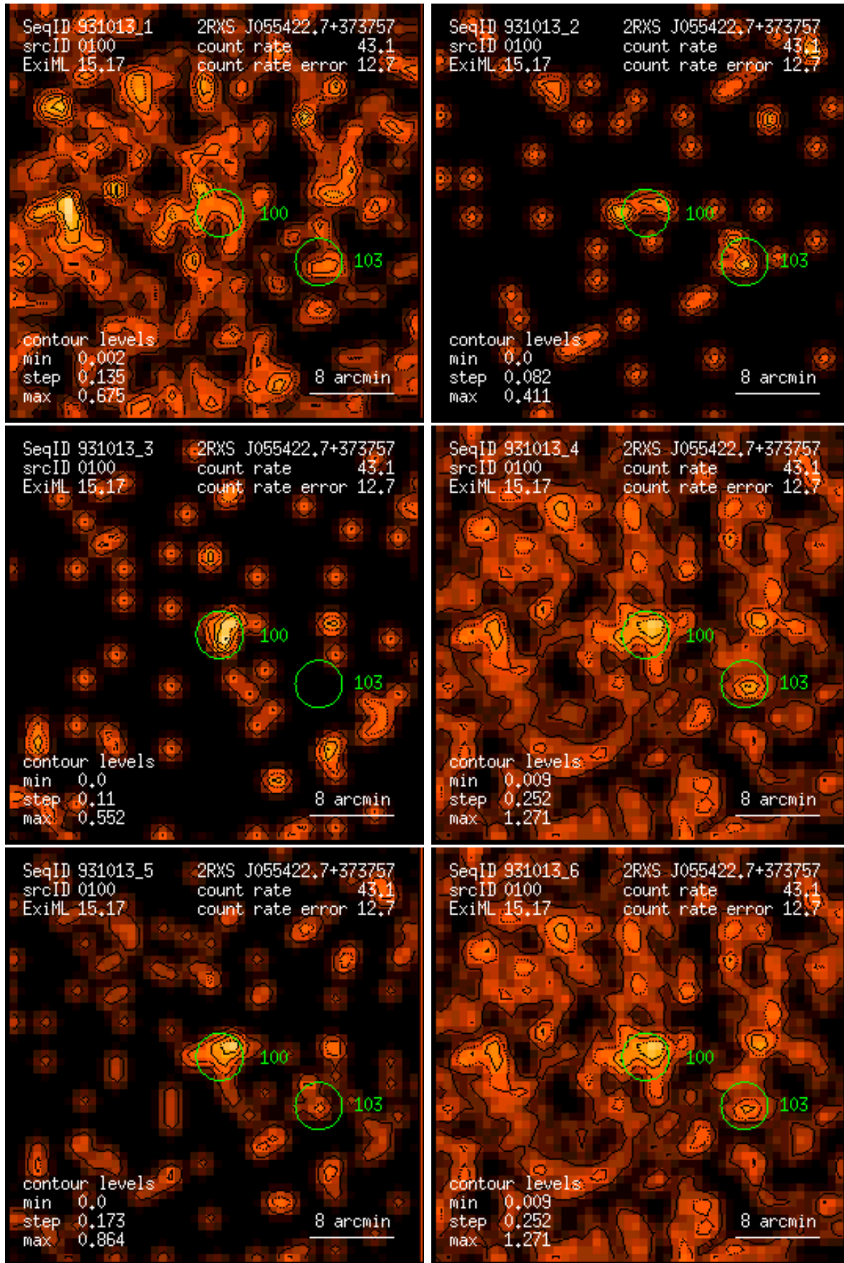
Figure 100: RASS 931013: detection 0100: band rate images, Gaussian filter: (1) PSPC channels 11 – 41, (2) 52 – 90, (3) 91 – 201, (4) 11 – 235, (5) 52 – 201, (6) 11 – 201. Broad band rates in counts/ks. Band rate contour levels in counts/ks/arcmin 2 .
