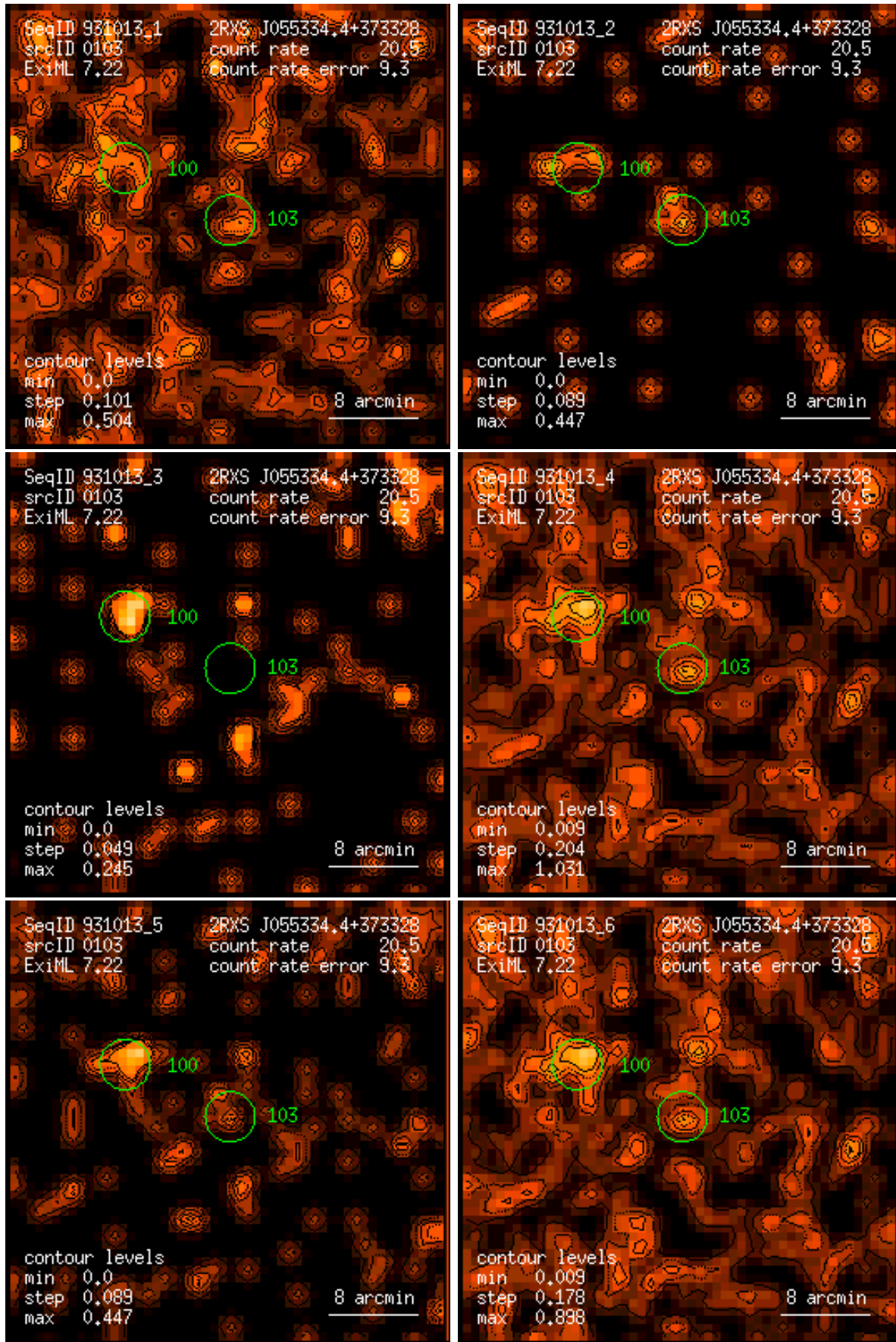
Figure 103: RASS 931013: detection 0103: band rate images, Gaussian filter: (1) PSPC channels 11 – 41, (2) 52 – 90, (3) 91 – 201, (4) 11 – 235, (5) 52 – 201, (6) 11 – 201. Broad band rates in counts/ks. Band rate contour levels in counts/ks/arcmin 2 .
