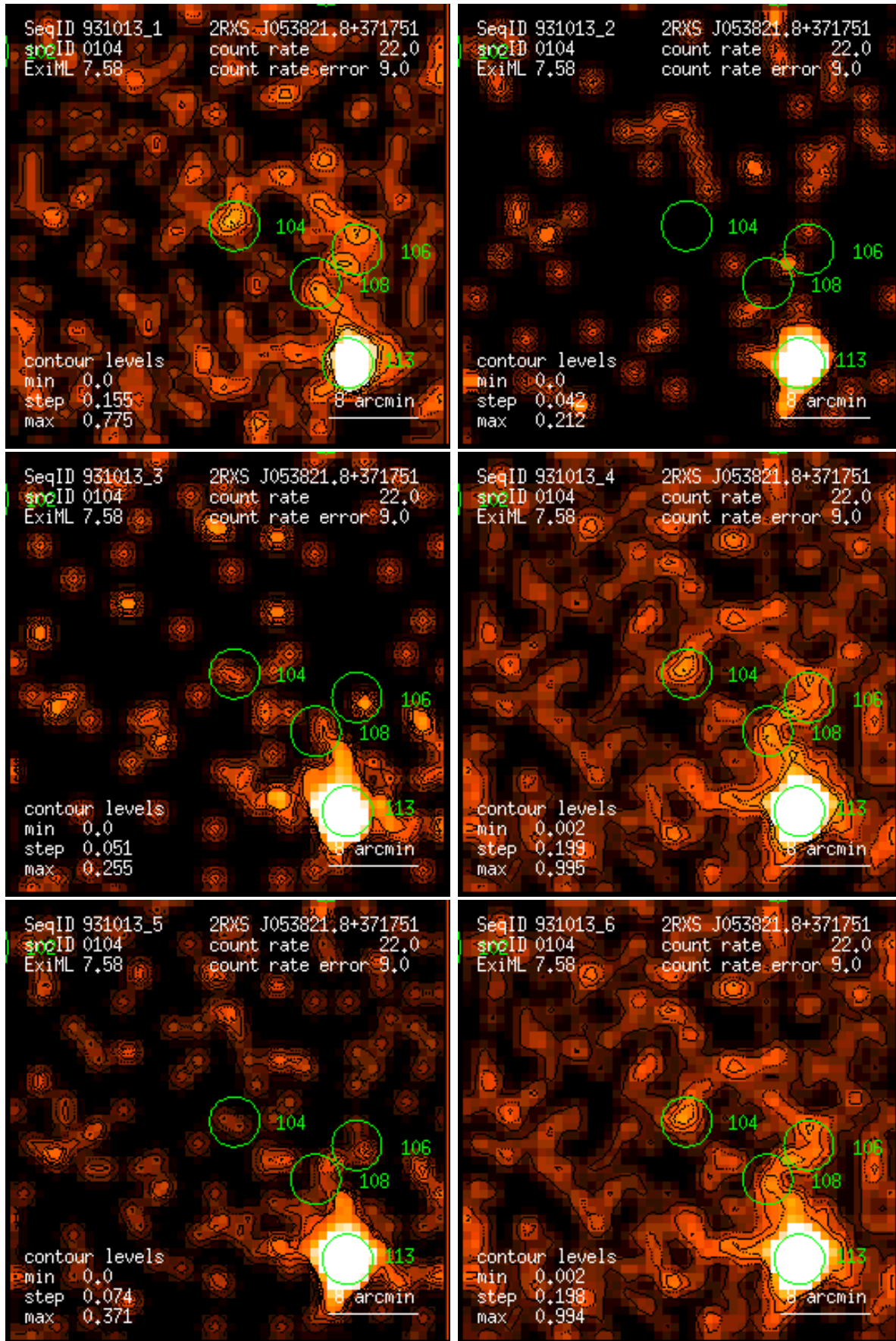
Figure 104: RASS 931013: detection 0104: band rate images, Gaussian filter: (1) PSPC channels 11 – 41, (2) 52 – 90, (3) 91 – 201, (4) 11 – 235, (5) 52 – 201, (6) 11 – 201. Broad band rates in counts/ks. Band rate contour levels in counts/ks/arcmin 2 .
