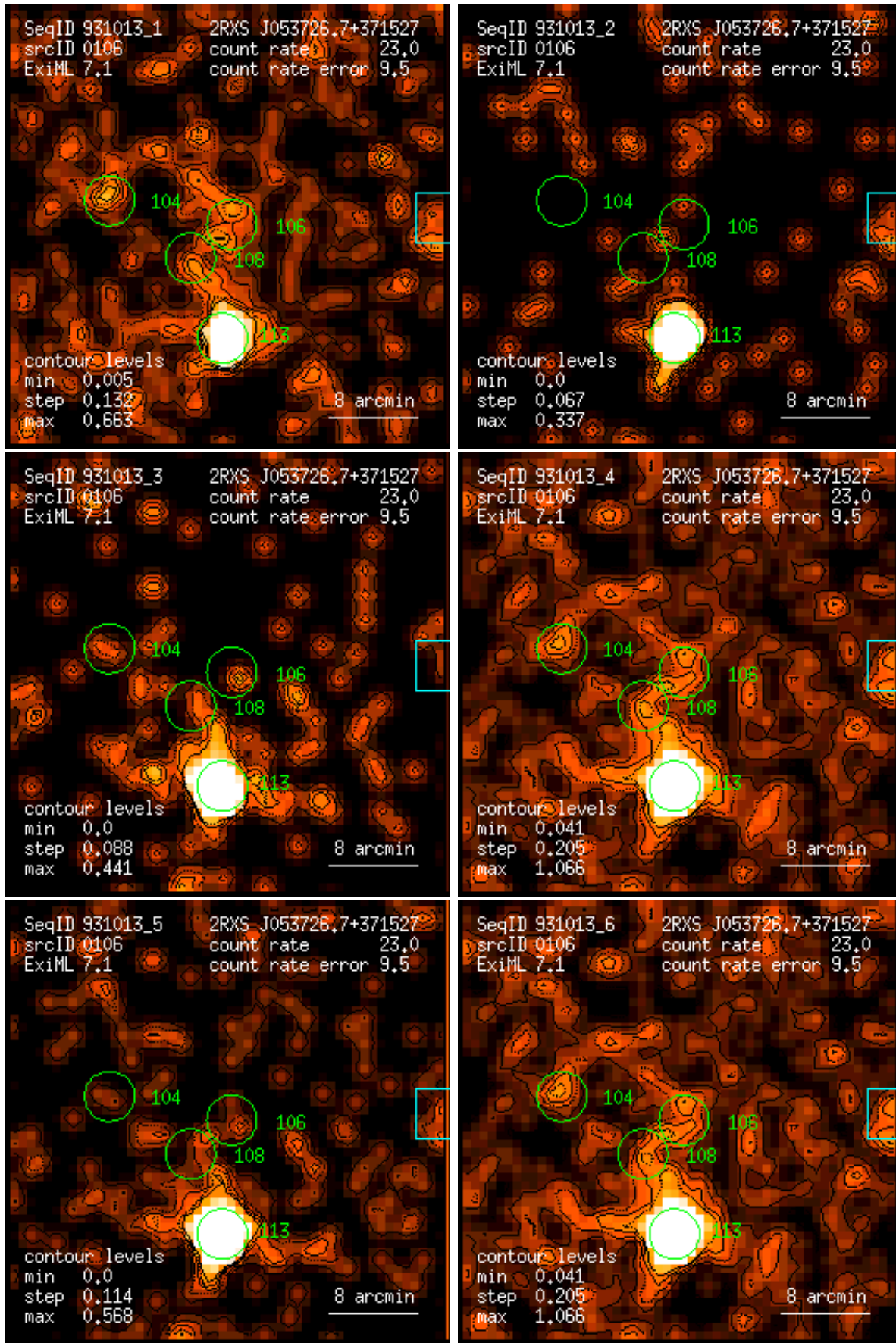
Figure 106: RASS 931013: detection 0106: band rate images, Gaussian filter: (1) PSPC channels 11 – 41, (2) 52 – 90, (3) 91 – 201, (4) 11 – 235, (5) 52 – 201, (6) 11 – 201. Broad band rates in counts/ks. Band rate contour levels in counts/ks/arcmin 2 .
