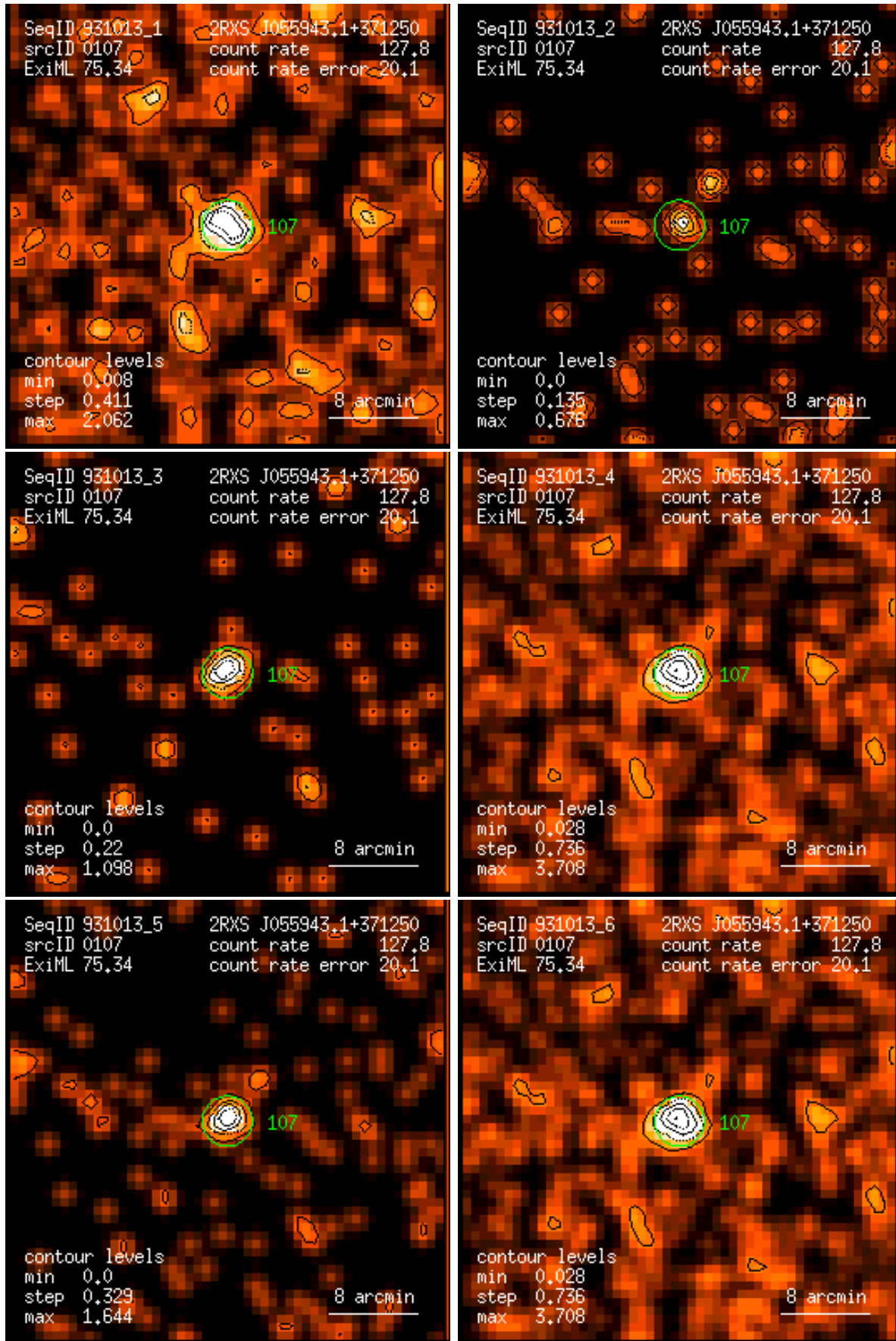
Figure 107: RASS 931013: detection 0107: band rate images, Gaussian filter: (1) PSPC channels 11 – 41, (2) 52 – 90, (3) 91 – 201, (4) 11 – 235, (5) 52 – 201, (6) 11 – 201. Broad band rates in counts/ks. Band rate contour levels in counts/ks/arcmin 2 .
