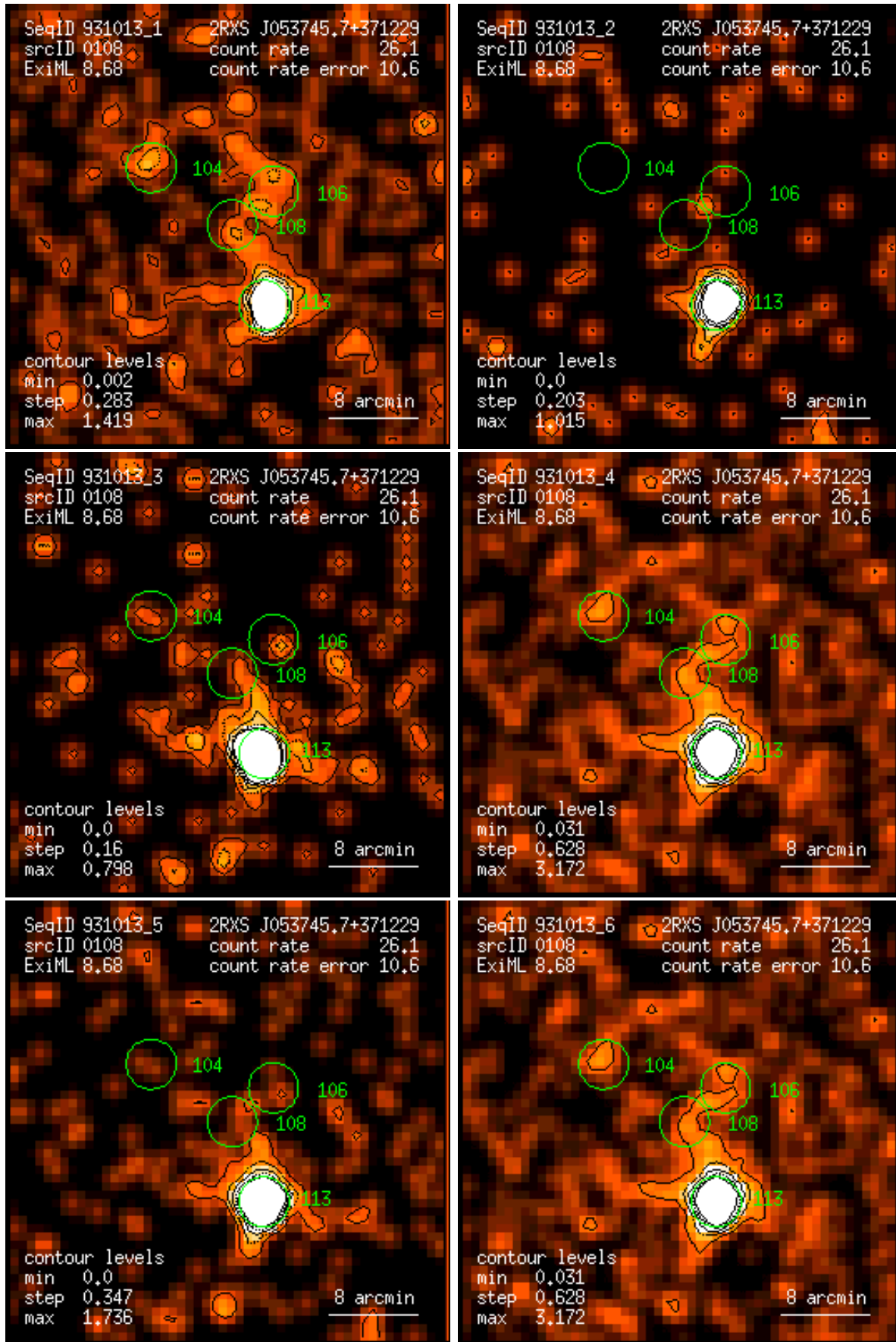
Figure 108: RASS 931013: detection 0108: band rate images, Gaussian filter: (1) PSPC channels 11 – 41, (2) 52 – 90, (3) 91 – 201, (4) 11 – 235, (5) 52 – 201, (6) 11 – 201. Broad band rates in counts/ks. Band rate contour levels in counts/ks/arcmin 2 .
