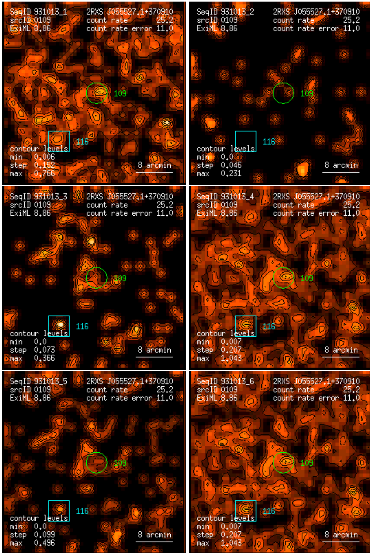
Figure 109: RASS 931013: detection 0109: band rate images, Gaussian filter: (1) PSPC channels 11 – 41, (2) 52 – 90, (3) 91 – 201, (4) 11 – 235, (5) 52 – 201, (6) 11 – 201. Broad band rates in counts/ks. Band rate contour levels in counts/ks/arcmin 2 .
