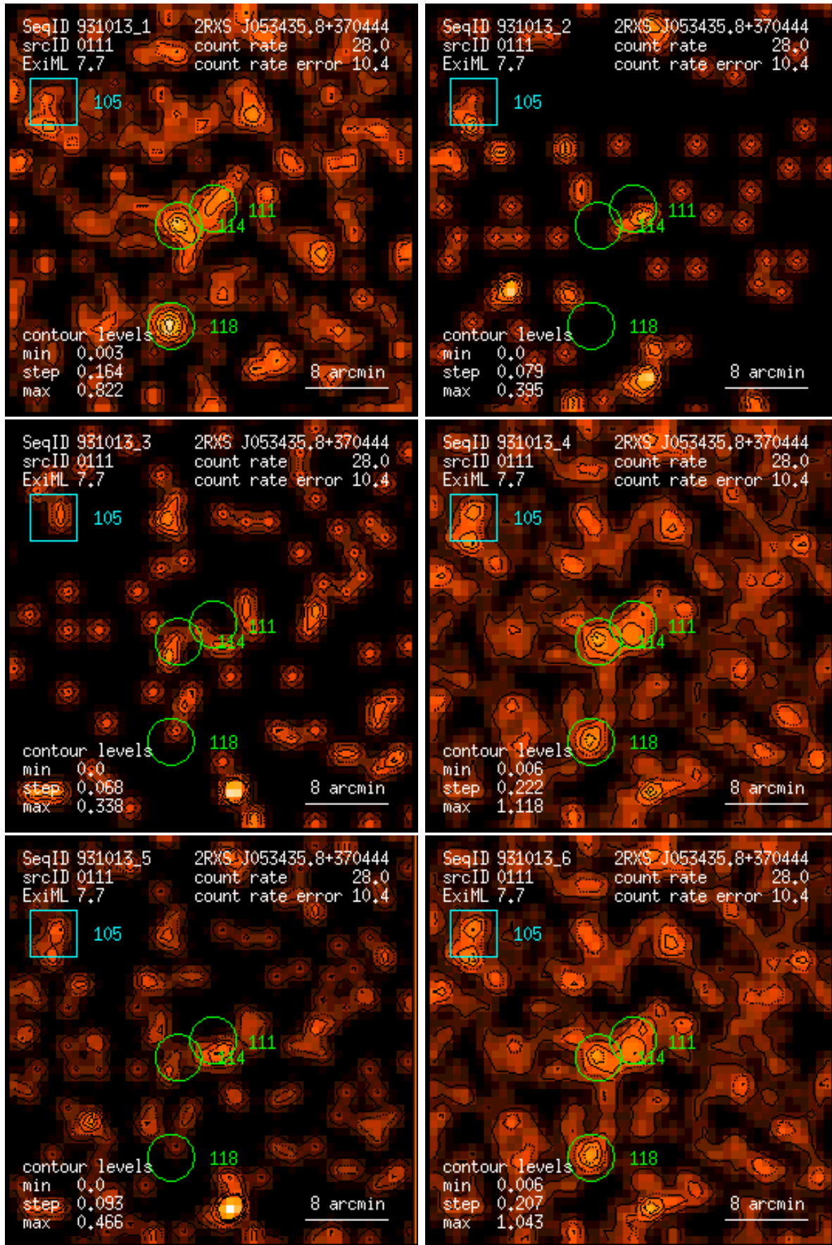
Figure 111: RASS 931013: detection 0111: band rate images, Gaussian filter: (1) PSPC channels 11 – 41, (2) 52 – 90, (3) 91 – 201, (4) 11 – 235, (5) 52 – 201, (6) 11 – 201. Broad band rates in counts/ks. Band rate contour levels in counts/ks/arcmin 2 .
