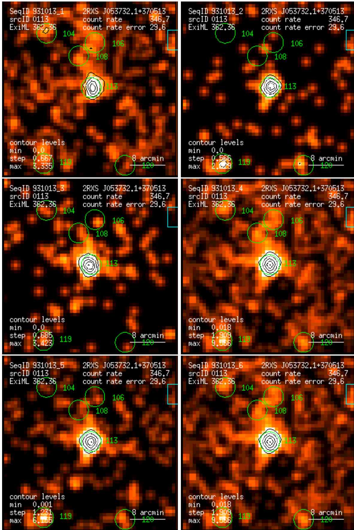
Figure 113: RASS 931013: detection 0113: band rate images, Gaussian filter: (1) PSPC channels 11 – 41, (2) 52 – 90, (3) 91 – 201, (4) 11 – 235, (5) 52 – 201, (6) 11 – 201. Broad band rates in counts/ks. Band rate contour levels in counts/ks/arcmin 2 .
